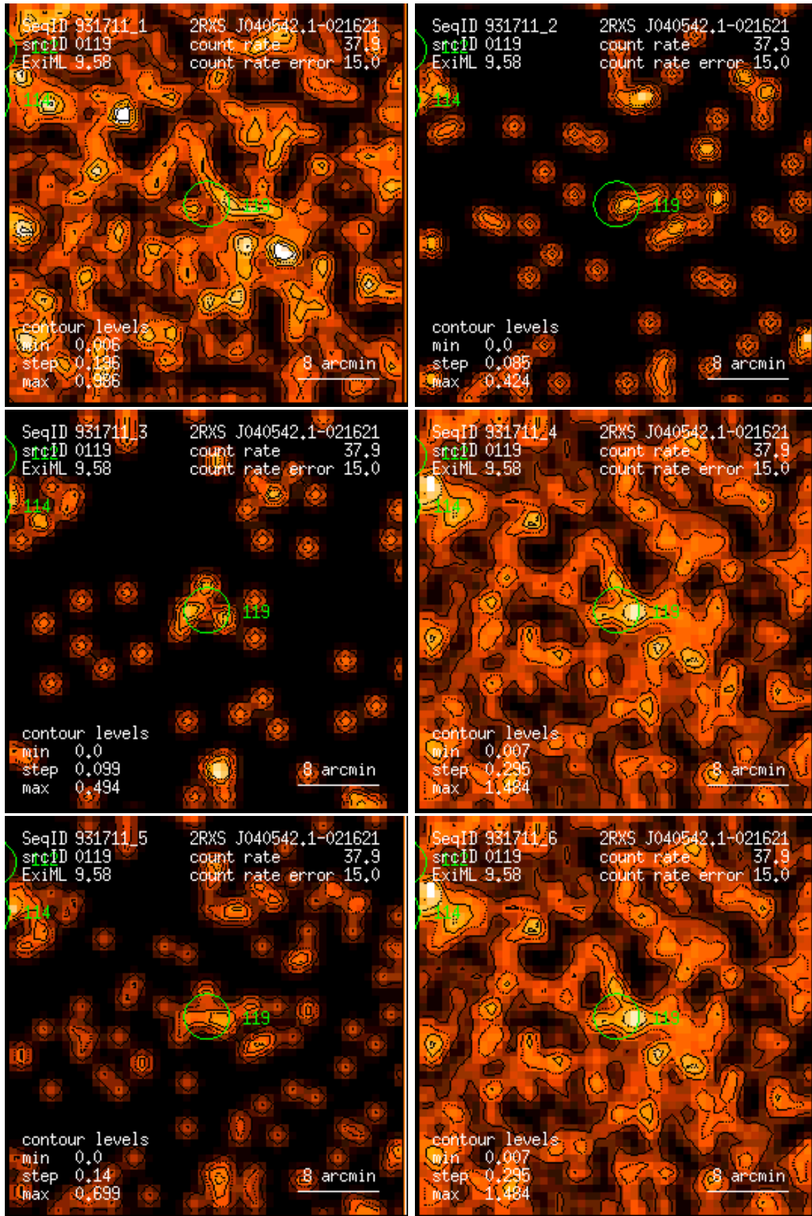
Figure 119: RASS 931711: detection 0119: band rate images, Gaussian filter: (1) PSPC channels 11 – 41, (2) 52 – 90, (3) 91 – 201, (4) 11 – 235, (5) 52 – 201, (6) 11 – 201. Broad band rates in counts/ks. Band rate contour levels in counts/ks/arcmin 2 .
