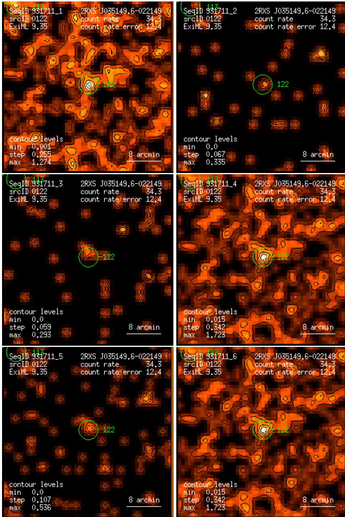
Figure 122: RASS 931711: detection 0122: band rate images, Gaussian filter: (1) PSPC channels 11 – 41, (2) 52 – 90, (3) 91 – 201, (4) 11 – 235, (5) 52 – 201, (6) 11 – 201. Broad band rates in counts/ks. Band rate contour levels in counts/ks/arcmin 2 .
