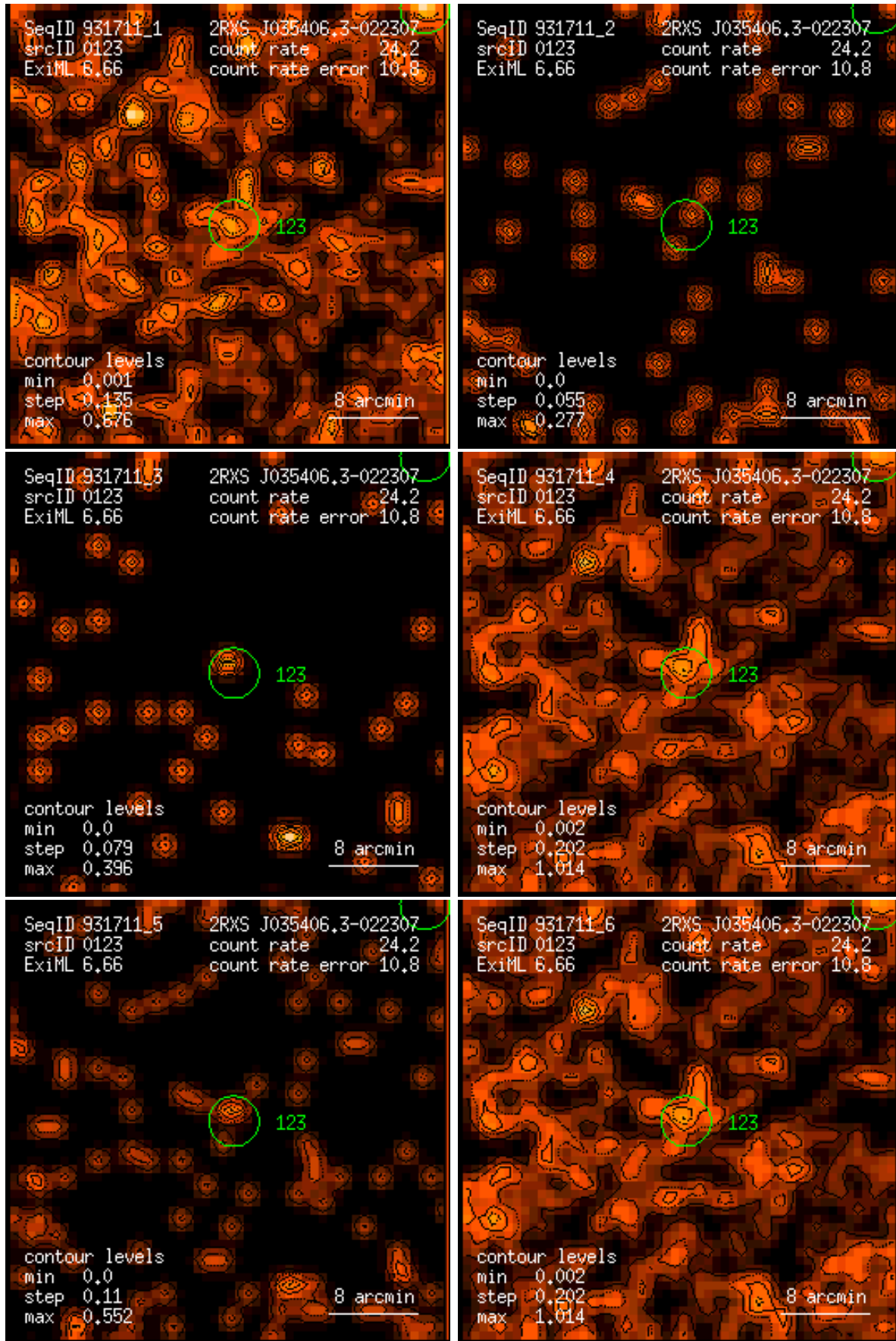
Figure 123: RASS 931711: detection 0123: band rate images, Gaussian filter: (1) PSPC channels 11 – 41, (2) 52 – 90, (3) 91 – 201, (4) 11 – 235, (5) 52 – 201, (6) 11 – 201. Broad band rates in counts/ks. Band rate contour levels in counts/ks/arcmin 2 .
