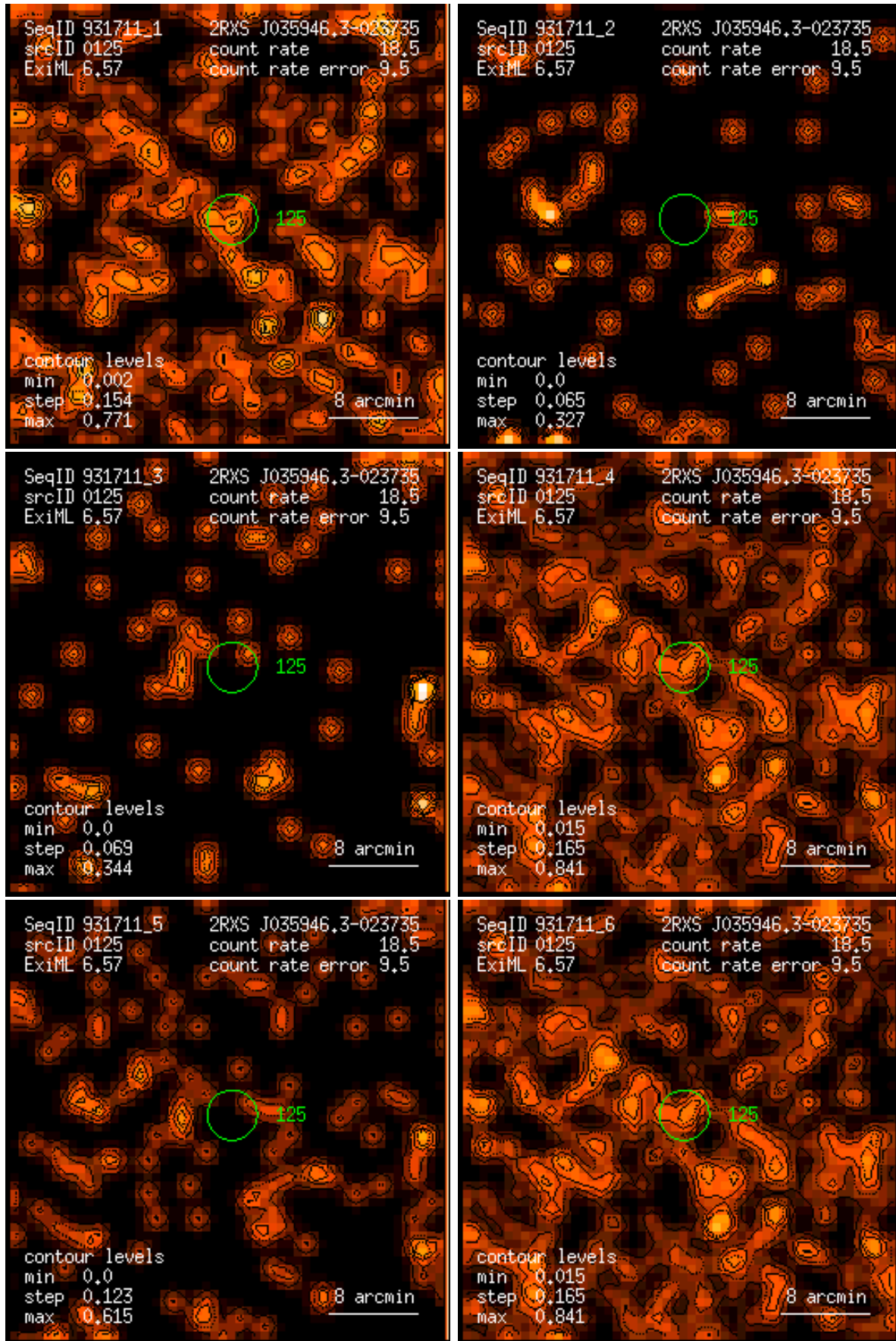
Figure 125: RASS 931711: detection 0125: band rate images, Gaussian filter: (1) PSPC channels 11 – 41, (2) 52 – 90, (3) 91 – 201, (4) 11 – 235, (5) 52 – 201, (6) 11 – 201. Broad band rates in counts/ks. Band rate contour levels in counts/ks/arcmin 2 .
