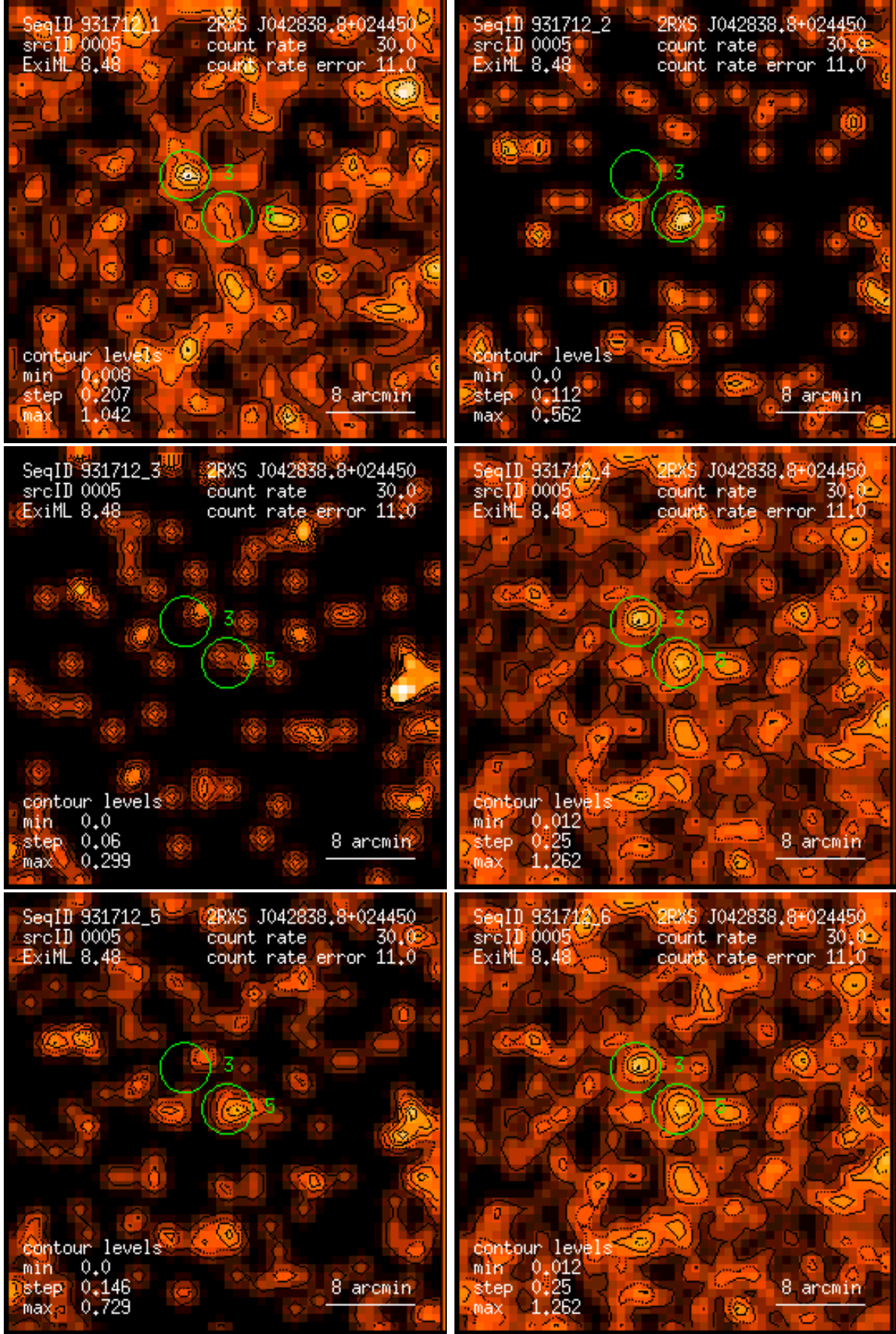
Figure 5: RASS 931712: detection 0005: band rate images, Gaussian filter: (1) PSPC channels 11 – 41, (2) 52 – 90, (3) 91 – 201, (4) 11 – 235, (5) 52 – 201, (6) 11 – 201. Broad band rates in counts/ks. Band rate contour levels in counts/ks/arcmin 2 .
