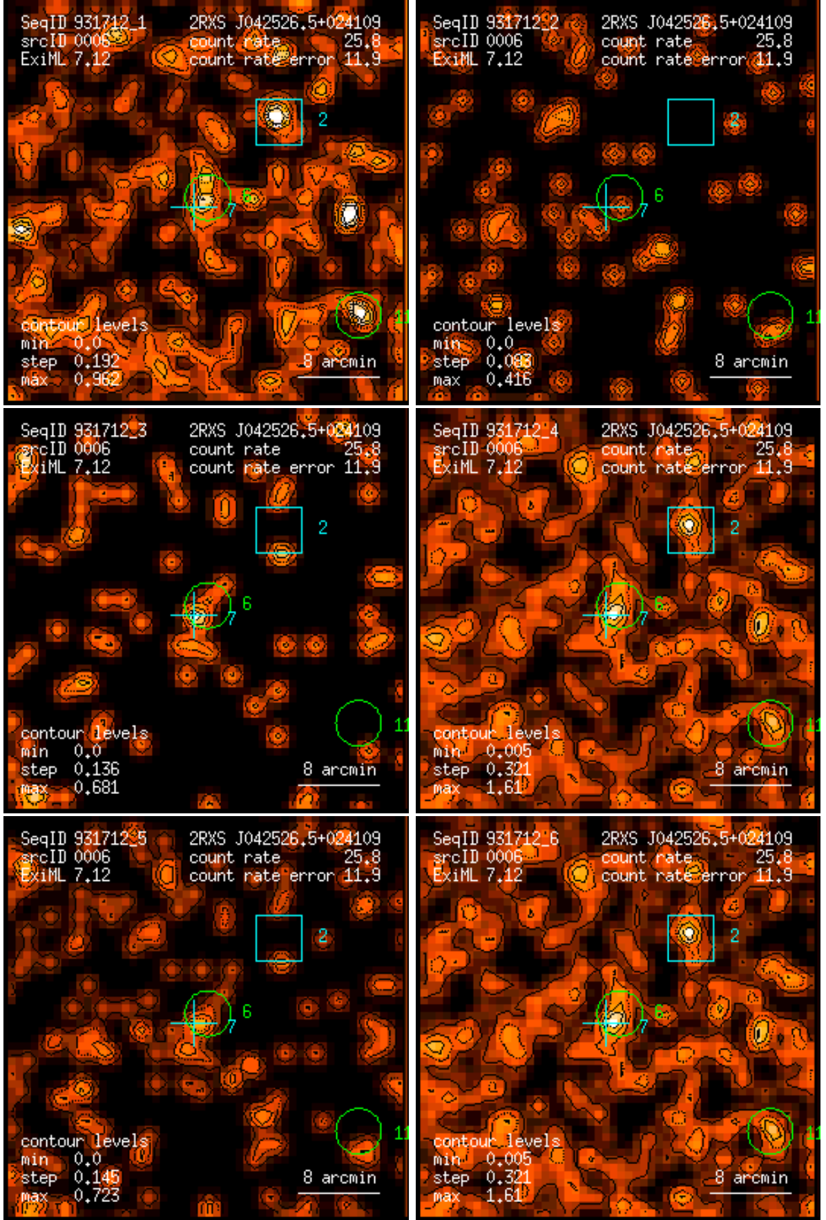
Figure 6: RASS 931712: detection 0006: band rate images, Gaussian filter: (1) PSPC channels 11 – 41, (2) 52 – 90, (3) 91 – 201, (4) 11 – 235, (5) 52 – 201, (6) 11 – 201. Broad band rates in counts/ks. Band rate contour levels in counts/ks/arcmin 2 .
