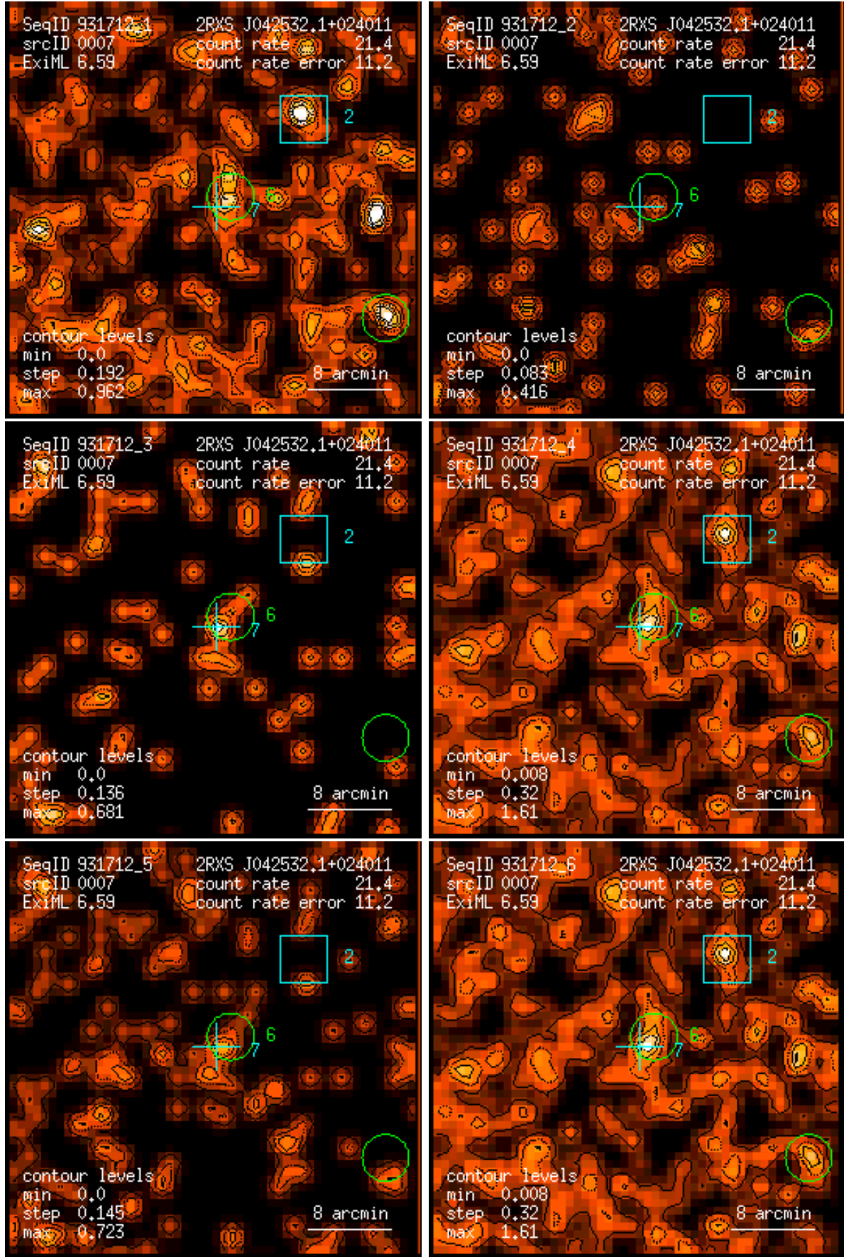
Figure 7: RASS 931712: detection 0007: band rate images, Gaussian filter: (1) PSPC channels 11 – 41, (2) 52 – 90, (3) 91 – 201, (4) 11 – 235, (5) 52 – 201, (6) 11 – 201. Broad band rates in counts/ks. Band rate contour levels in counts/ks/arcmin 2 .
