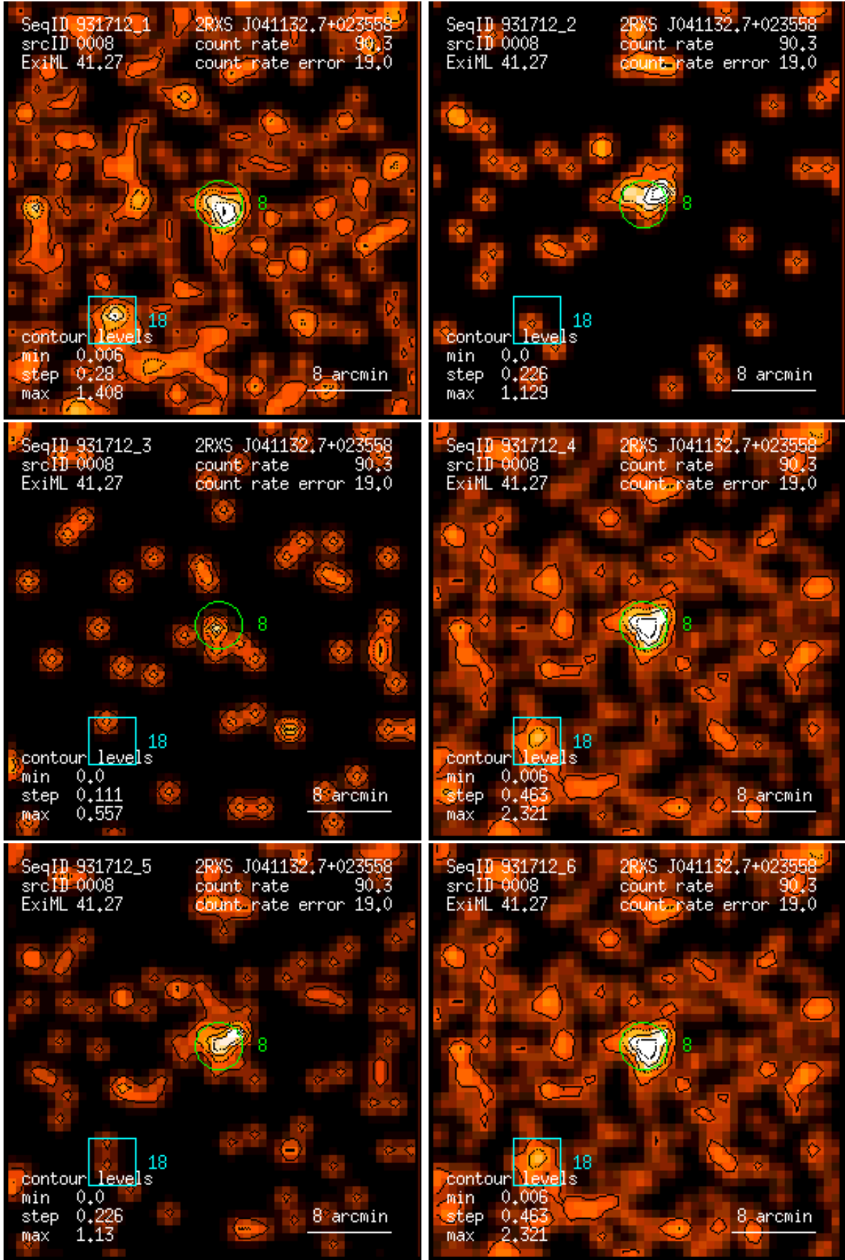
Figure 8: RASS 931712: detection 0008: band rate images, Gaussian filter: (1) PSPC channels 11 – 41, (2) 52 – 90, (3) 91 – 201, (4) 11 – 235, (5) 52 – 201, (6) 11 – 201. Broad band rates in counts/ks. Band rate contour levels in counts/ks/arcmin 2 .
