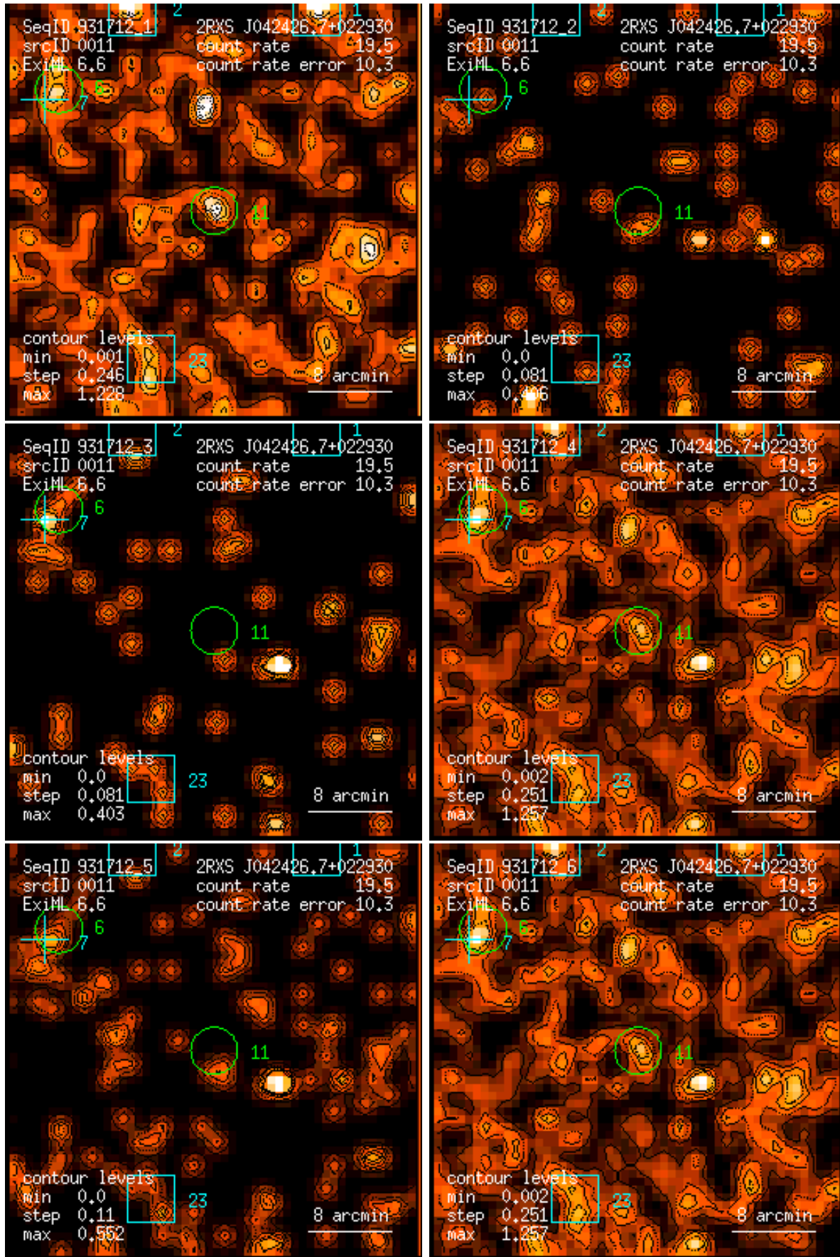
Figure 11: RASS 931712: detection 0011: band rate images, Gaussian filter: (1) PSPC channels 11 – 41, (2) 52 – 90, (3) 91 – 201, (4) 11 – 235, (5) 52 – 201, (6) 11 – 201. Broad band rates in counts/ks. Band rate contour levels in counts/ks/arcmin 2 .
