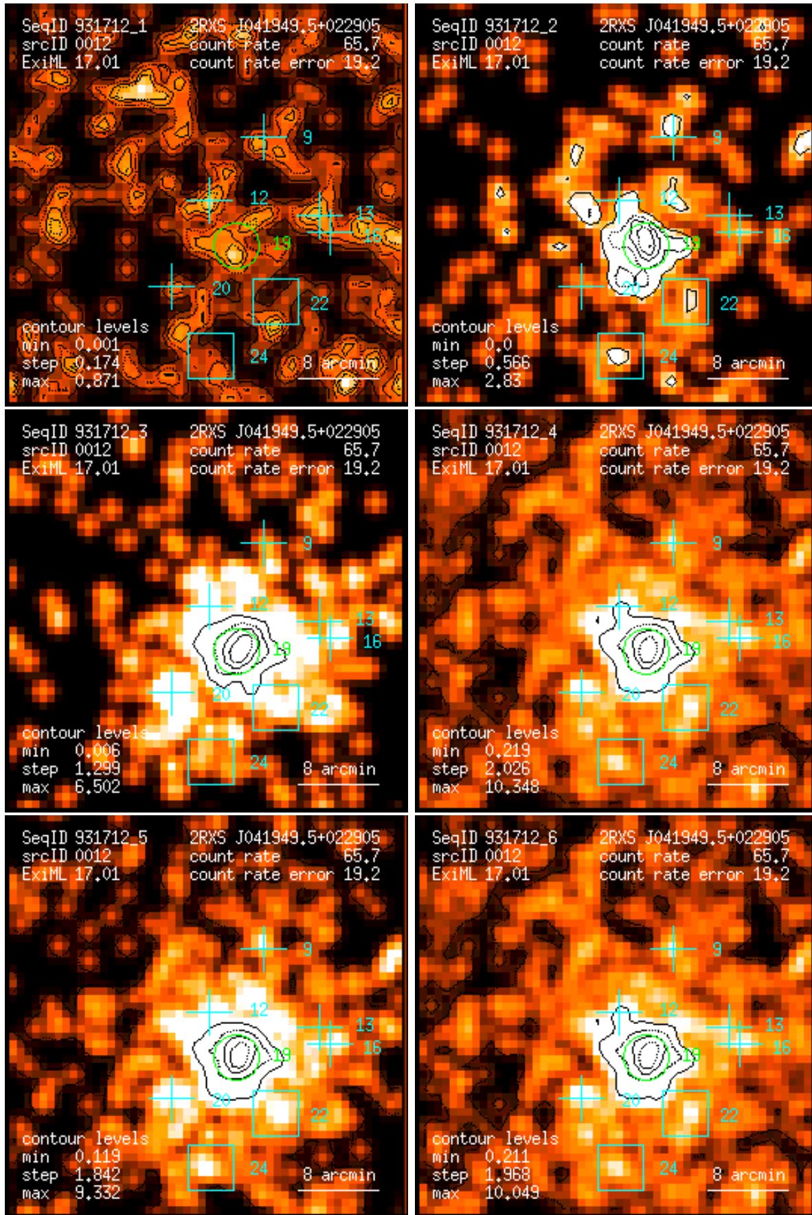
Figure 12: RASS 931712: detection 0012: band rate images, Gaussian filter: (1) PSPC channels 11 – 41, (2) 52 – 90, (3) 91 – 201, (4) 11 – 235, (5) 52 – 201, (6) 11 – 201. Broad band rates in counts/ks. Band rate contour levels in counts/ks/arcmin 2 .
