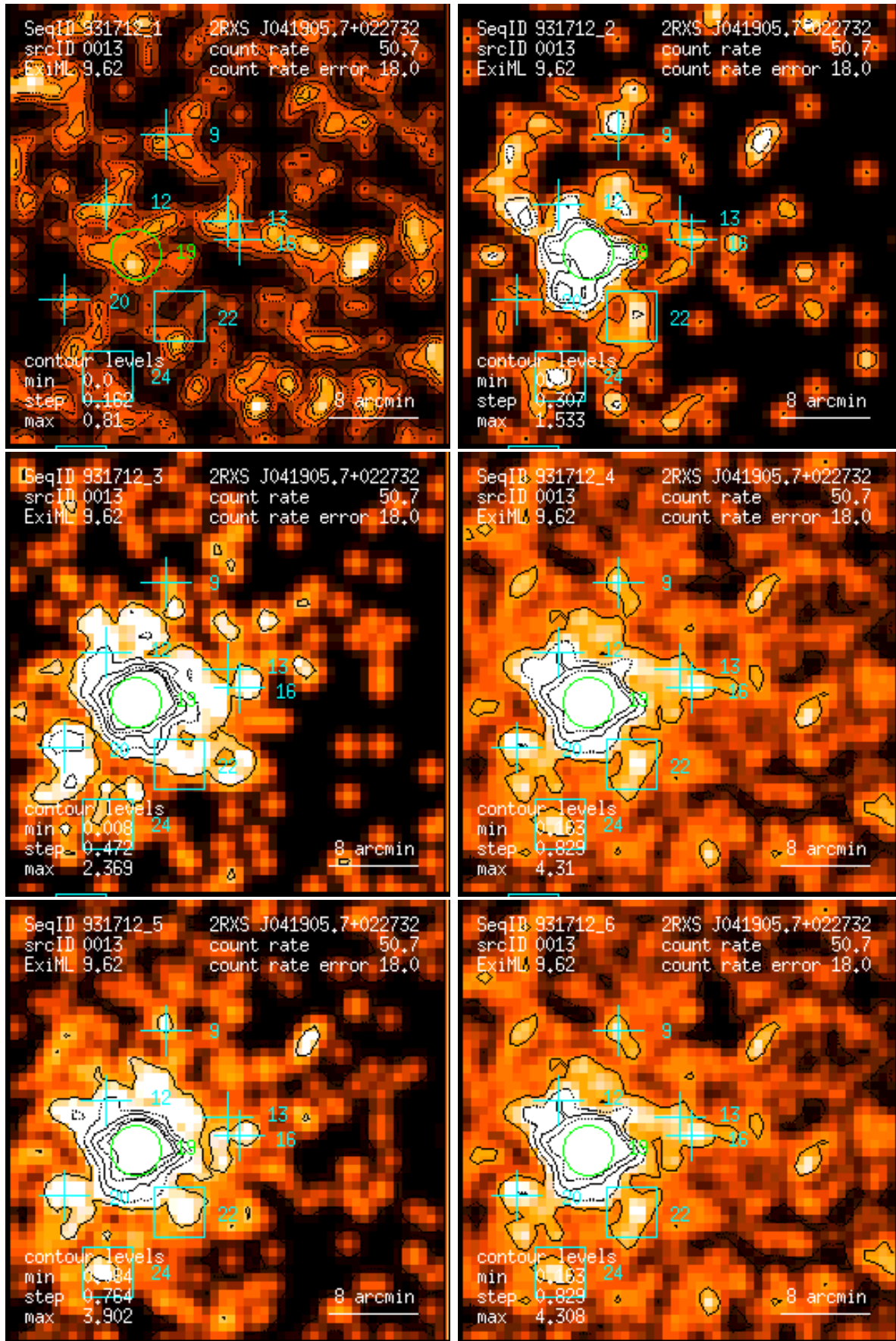
Figure 13: RASS 931712: detection 0013: band rate images, Gaussian filter: (1) PSPC channels 11 – 41, (2) 52 – 90, (3) 91 – 201, (4) 11 – 235, (5) 52 – 201, (6) 11 – 201. Broad band rates in counts/ks. Band rate contour levels in counts/ks/arcmin 2 .
