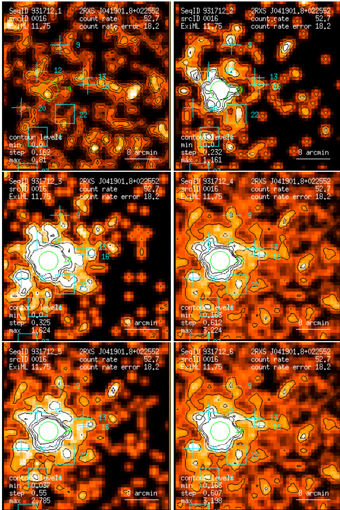
Figure 16: RASS 931712: detection 0016: band rate images, Gaussian filter: (1) PSPC channels 11 – 41, (2) 52 – 90, (3) 91 – 201, (4) 11 – 235, (5) 52 – 201, (6) 11 – 201. Broad band rates in counts/ks. Band rate contour levels in counts/ks/arcmin 2 .
