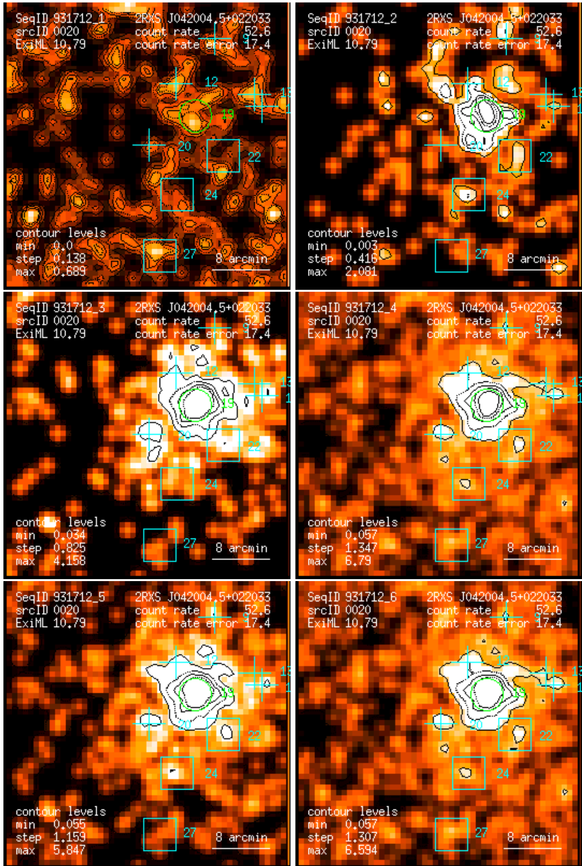
Figure 20: RASS 931712: detection 0020: band rate images, Gaussian filter: (1) PSPC channels 11 – 41, (2) 52 – 90, (3) 91 – 201, (4) 11 – 235, (5) 52 – 201, (6) 11 – 201. Broad band rates in counts/ks. Band rate contour levels in counts/ks/arcmin 2 .
