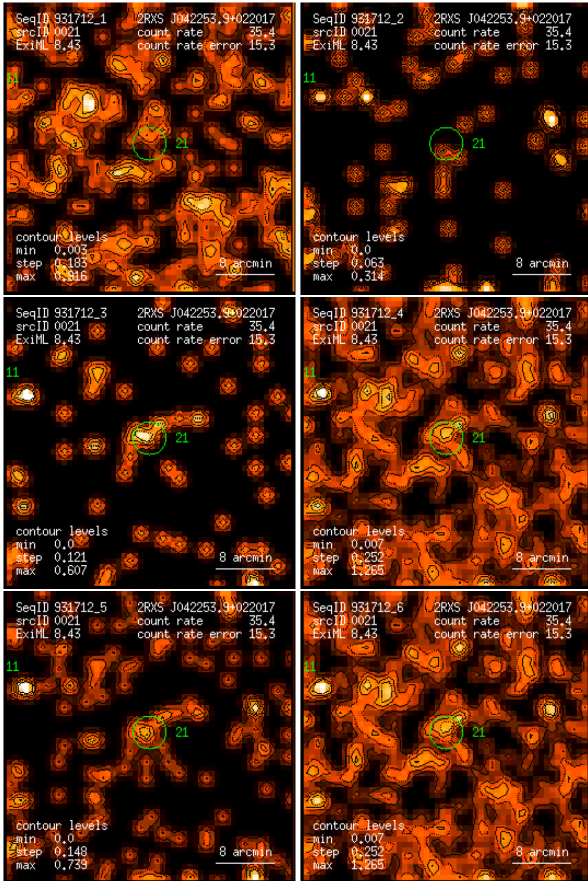
Figure 21: RASS 931712: detection 0021: band rate images, Gaussian filter: (1) PSPC channels 11 – 41, (2) 52 – 90, (3) 91 – 201, (4) 11 – 235, (5) 52 – 201, (6) 11 – 201. Broad band rates in counts/ks. Band rate contour levels in counts/ks/arcmin 2 .
