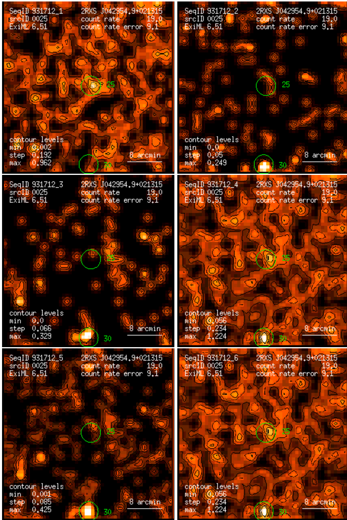
Figure 25: RASS 931712: detection 0025: band rate images, Gaussian filter: (1) PSPC channels 11 – 41, (2) 52 – 90, (3) 91 – 201, (4) 11 – 235, (5) 52 – 201, (6) 11 – 201. Broad band rates in counts/ks. Band rate contour levels in counts/ks/arcmin 2 .
