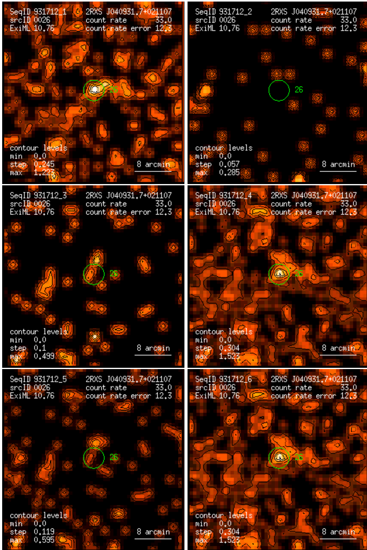
Figure 26: RASS 931712: detection 0026: band rate images, Gaussian filter: (1) PSPC channels 11 – 41, (2) 52 – 90, (3) 91 – 201, (4) 11 – 235, (5) 52 – 201, (6) 11 – 201. Broad band rates in counts/ks. Band rate contour levels in counts/ks/arcmin 2 .
