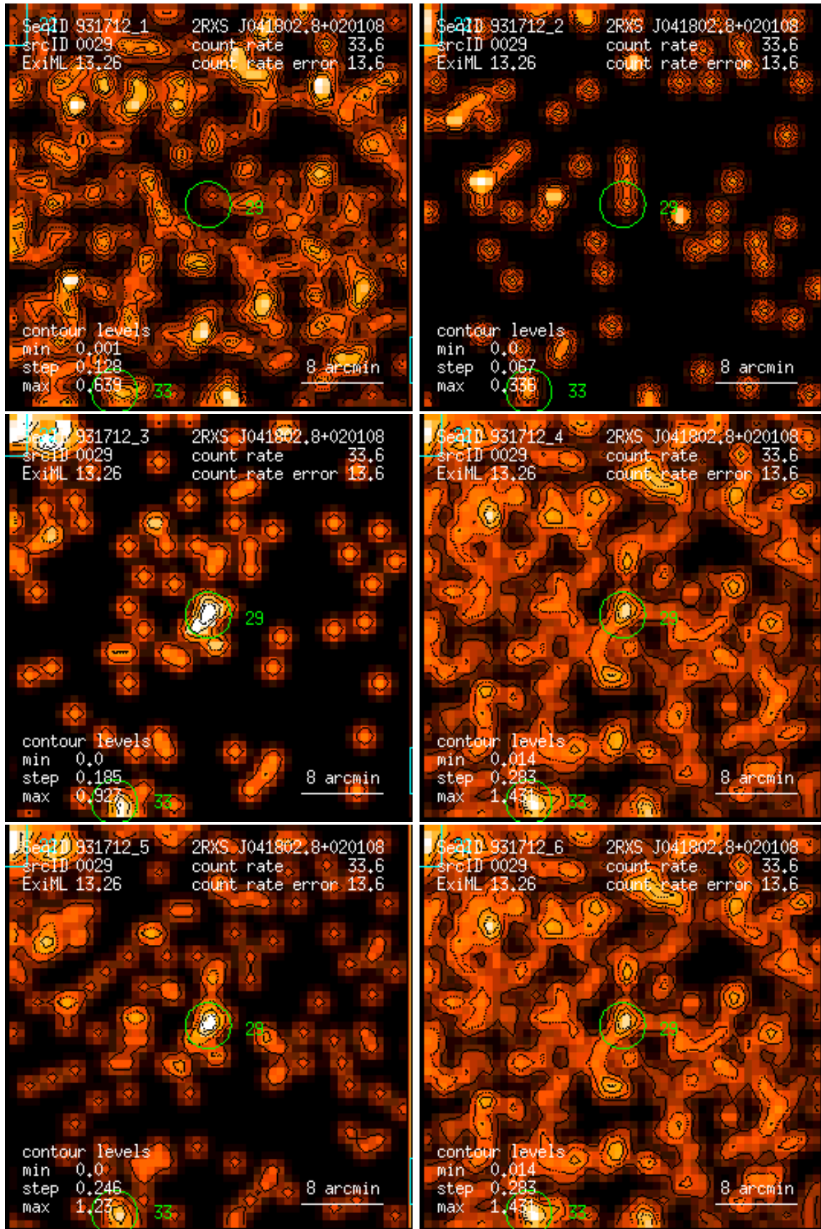
Figure 29: RASS 931712: detection 0029: band rate images, Gaussian filter: (1) PSPC channels 11 – 41, (2) 52 – 90, (3) 91 – 201, (4) 11 – 235, (5) 52 – 201, (6) 11 – 201. Broad band rates in counts/ks. Band rate contour levels in counts/ks/arcmin 2 .
