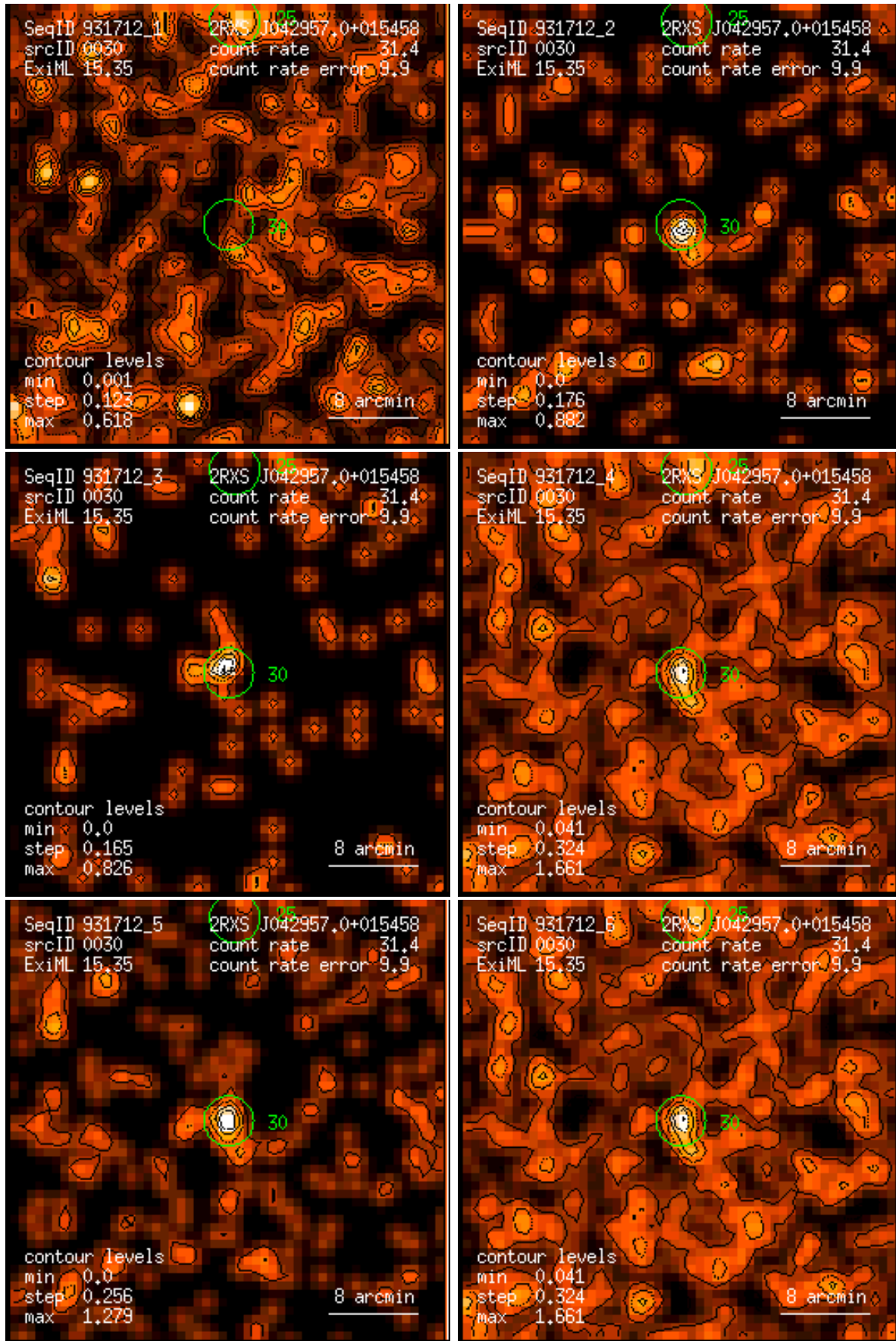
Figure 30: RASS 931712: detection 0030: band rate images, Gaussian filter: (1) PSPC channels 11 – 41, (2) 52 – 90, (3) 91 – 201, (4) 11 – 235, (5) 52 – 201, (6) 11 – 201. Broad band rates in counts/ks. Band rate contour levels in counts/ks/arcmin 2 .
