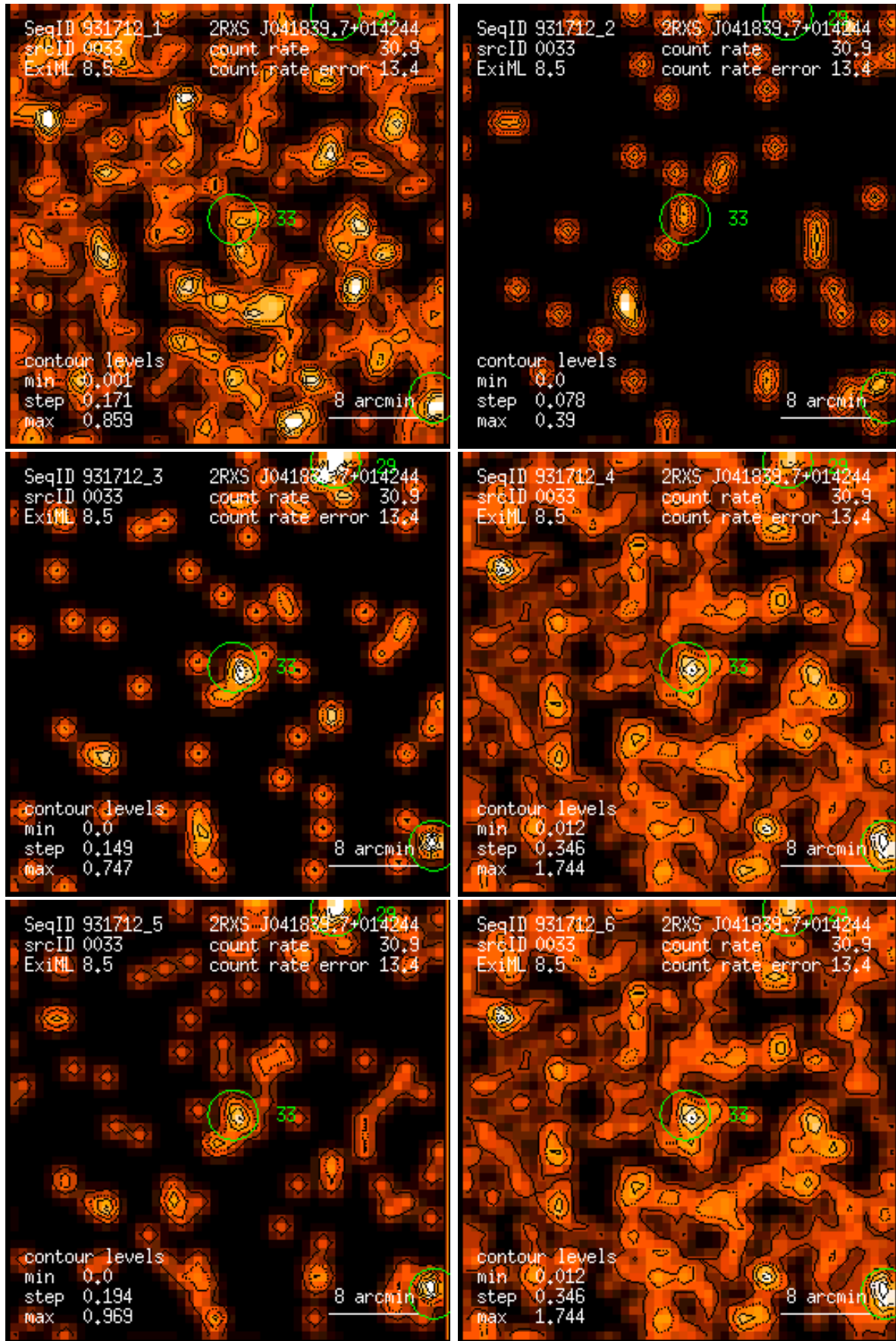
Figure 33: RASS 931712: detection 0033: band rate images, Gaussian filter: (1) PSPC channels 11 – 41, (2) 52 – 90, (3) 91 – 201, (4) 11 – 235, (5) 52 – 201, (6) 11 – 201. Broad band rates in counts/ks. Band rate contour levels in counts/ks/arcmin 2 .
