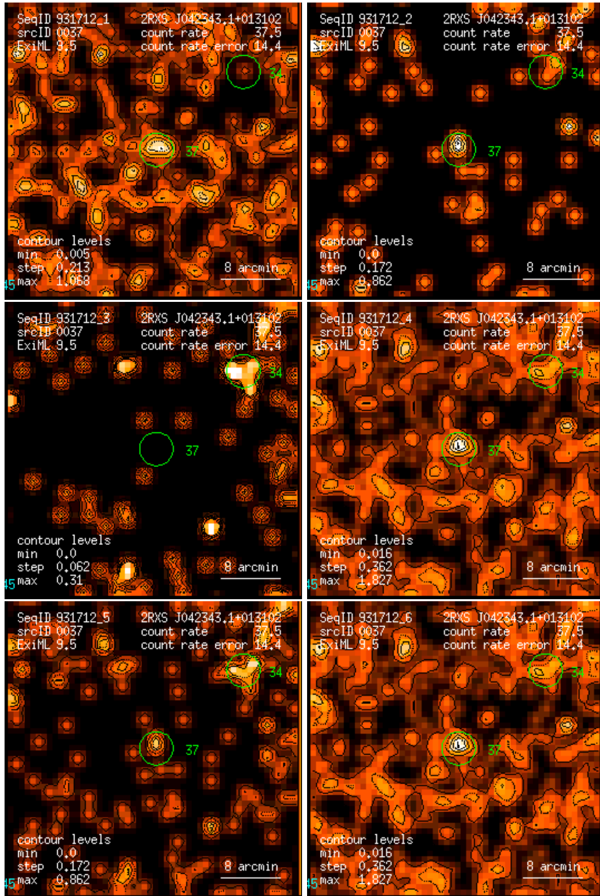
Figure 37: RASS 931712: detection 0037: band rate images, Gaussian filter: (1) PSPC channels 11 – 41, (2) 52 – 90, (3) 91 – 201, (4) 11 – 235, (5) 52 – 201, (6) 11 – 201. Broad band rates in counts/ks. Band rate contour levels in counts/ks/arcmin 2 .
