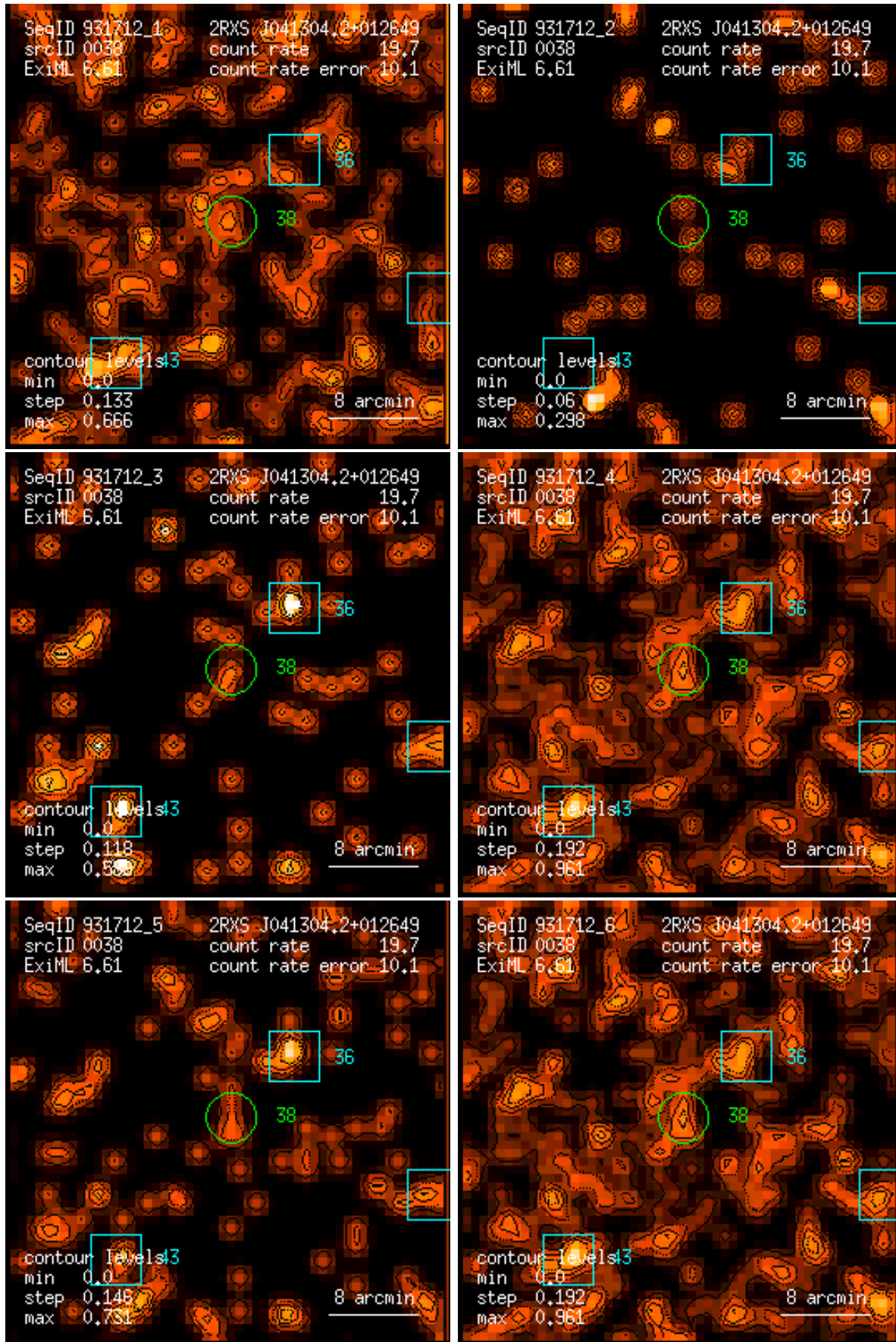
Figure 38: RASS 931712: detection 0038: band rate images, Gaussian filter: (1) PSPC channels 11 – 41, (2) 52 – 90, (3) 91 – 201, (4) 11 – 235, (5) 52 – 201, (6) 11 – 201. Broad band rates in counts/ks. Band rate contour levels in counts/ks/arcmin 2 .
