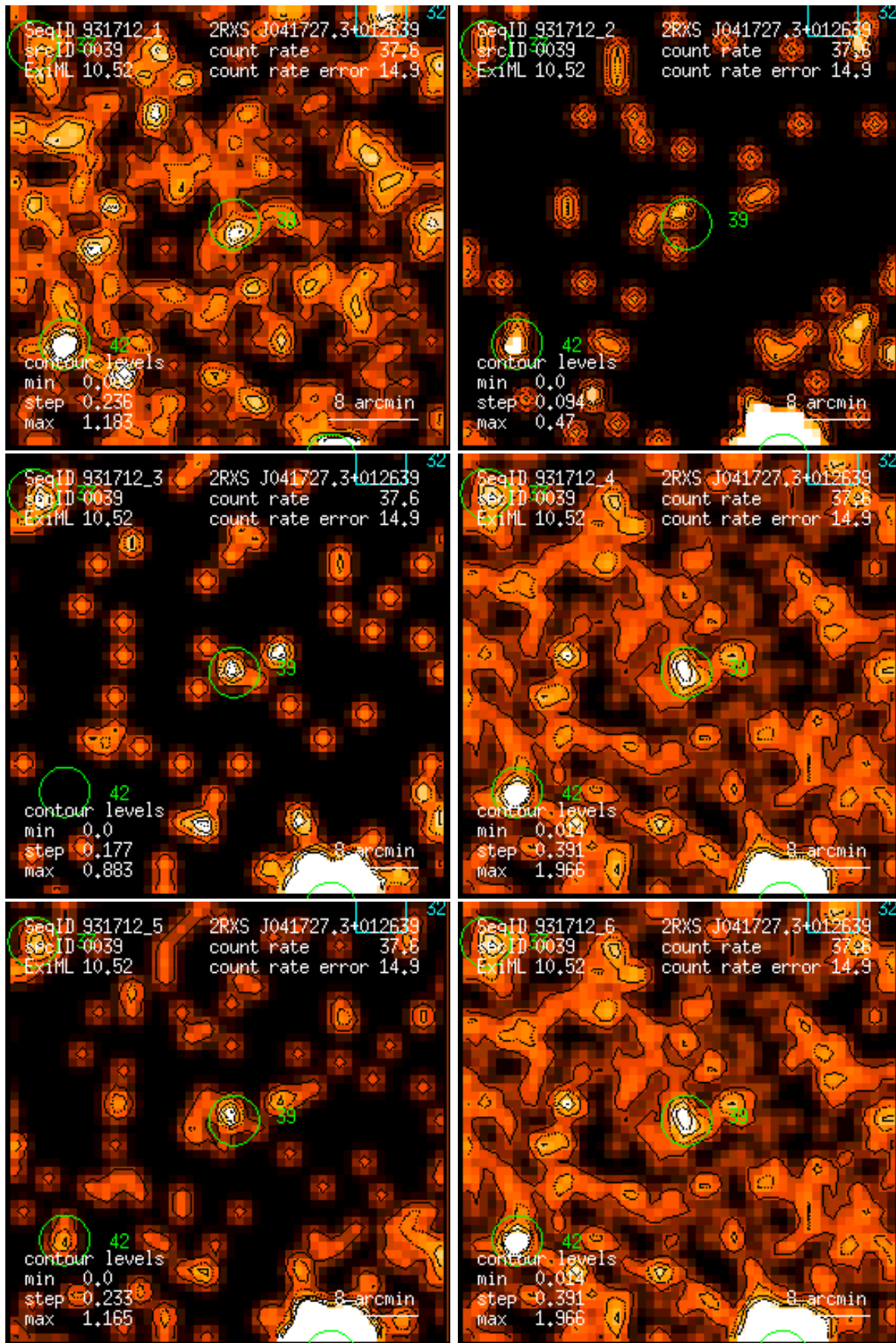
Figure 39: RASS 931712: detection 0039: band rate images, Gaussian filter: (1) PSPC channels 11 – 41, (2) 52 – 90, (3) 91 – 201, (4) 11 – 235, (5) 52 – 201, (6) 11 – 201. Broad band rates in counts/ks. Band rate contour levels in counts/ks/arcmin 2 .
