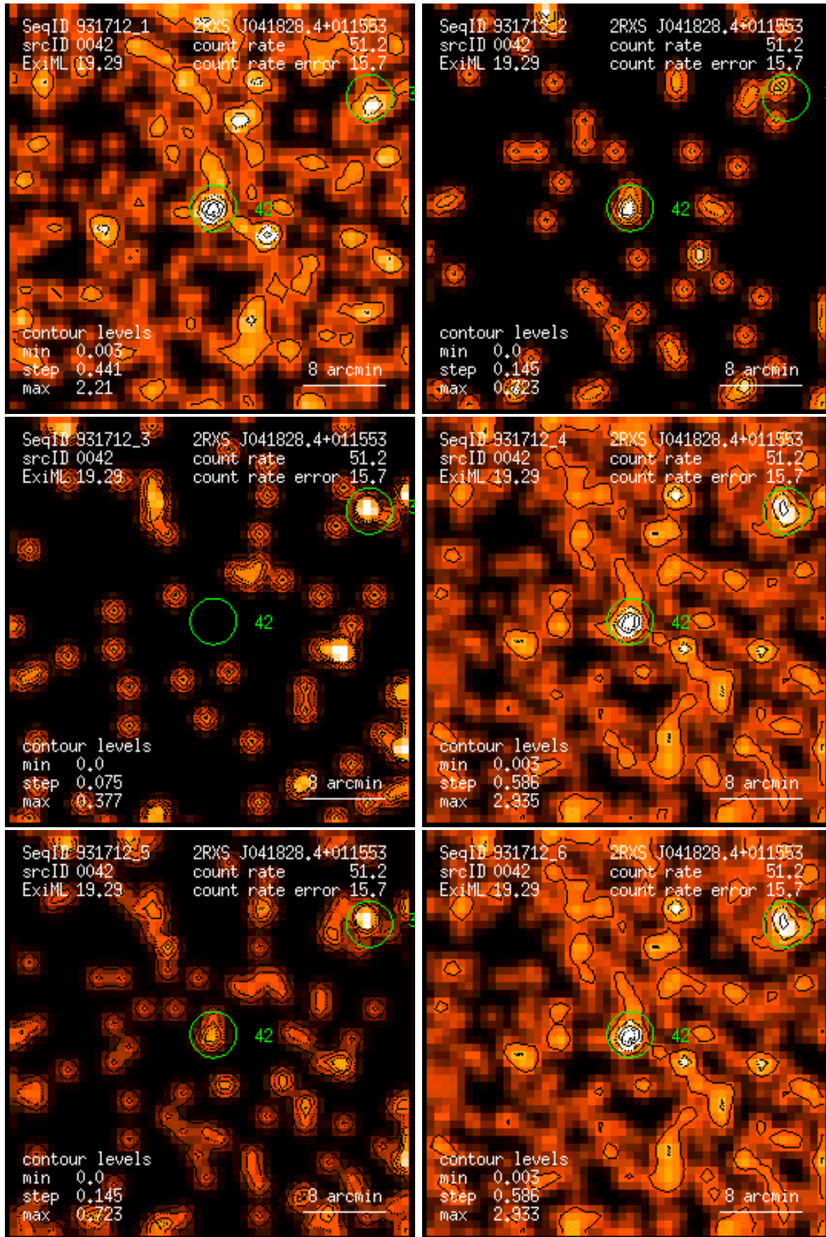
Figure 42: RASS 931712: detection 0042: band rate images, Gaussian filter: (1) PSPC channels 11 – 41, (2) 52 – 90, (3) 91 – 201, (4) 11 – 235, (5) 52 – 201, (6) 11 – 201. Broad band rates in counts/ks. Band rate contour levels in counts/ks/arcmin 2 .
