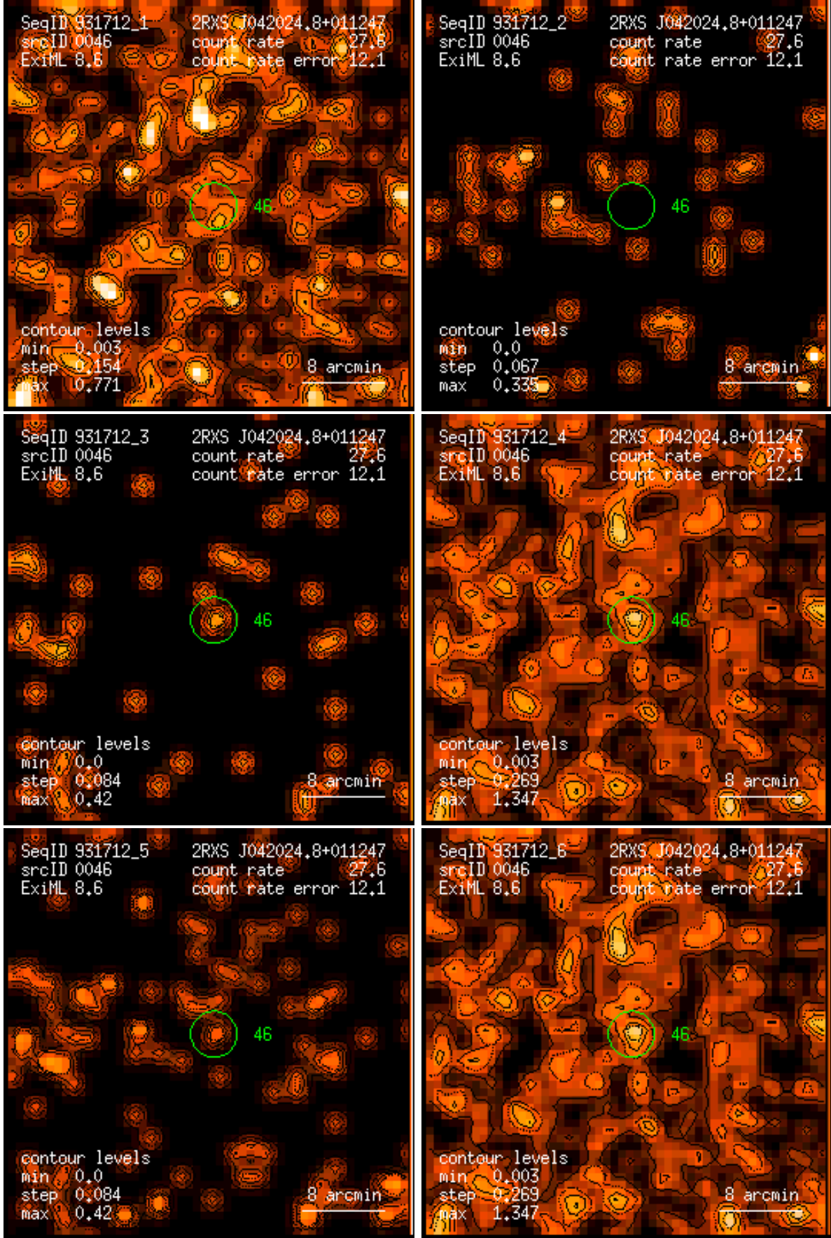
Figure 46: RASS 931712: detection 0046: band rate images, Gaussian filter: (1) PSPC channels 11 – 41, (2) 52 – 90, (3) 91 – 201, (4) 11 – 235, (5) 52 – 201, (6) 11 – 201. Broad band rates in counts/ks. Band rate contour levels in counts/ks/arcmin 2 .
