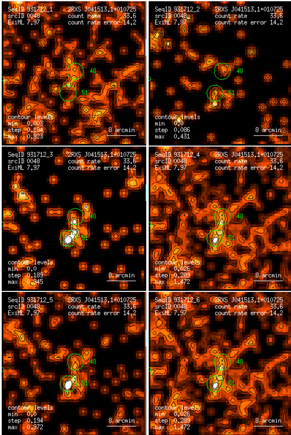
Figure 48: RASS 931712: detection 0048: band rate images, Gaussian filter: (1) PSPC channels 11 – 41, (2) 52 – 90, (3) 91 – 201, (4) 11 – 235, (5) 52 – 201, (6) 11 – 201. Broad band rates in counts/ks. Band rate contour levels in counts/ks/arcmin 2 .
