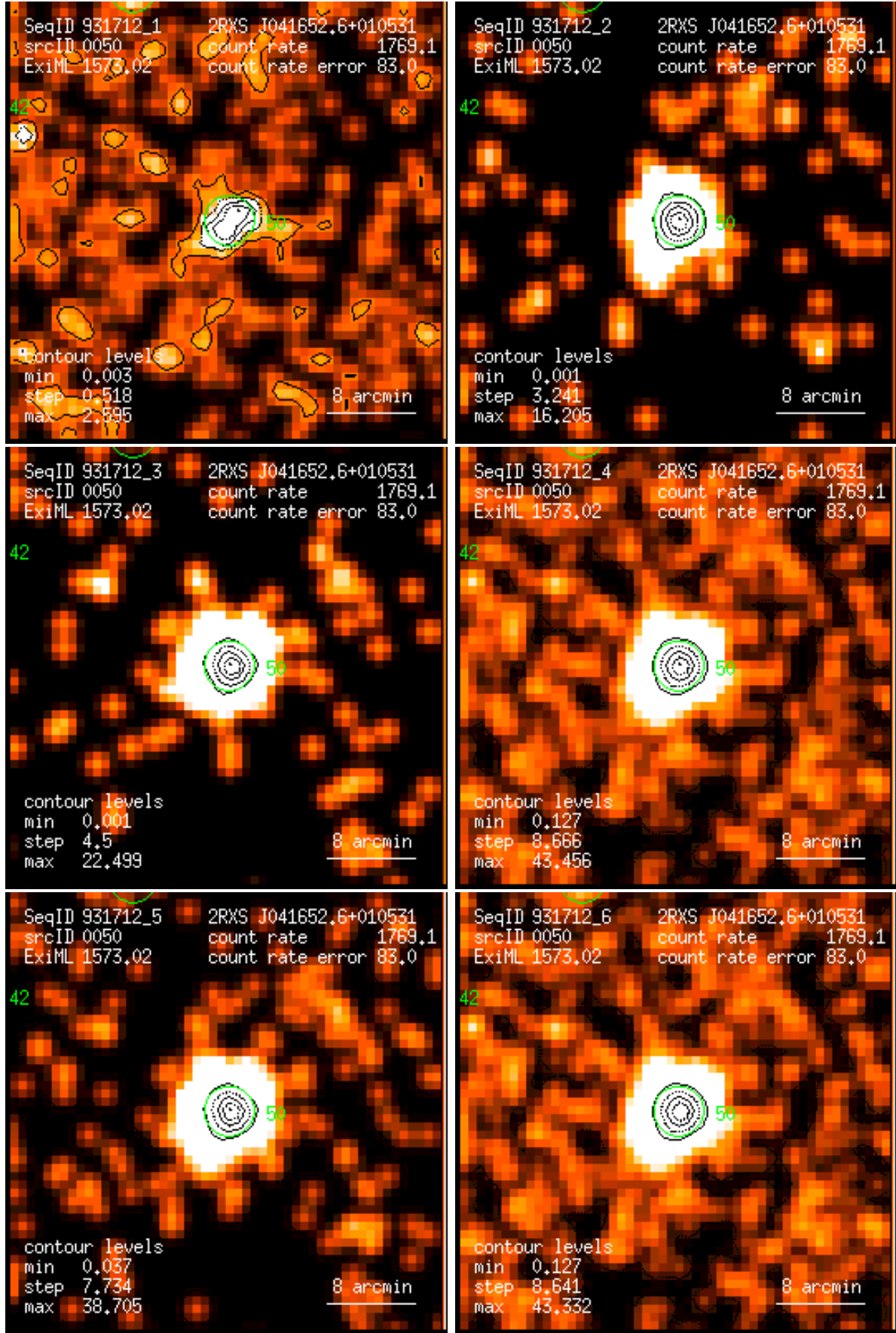
Figure 50: RASS 931712: detection 0050: band rate images, Gaussian filter: (1) PSPC channels 11 – 41, (2) 52 – 90, (3) 91 – 201, (4) 11 – 235, (5) 52 – 201, (6) 11 – 201. Broad band rates in counts/ks. Band rate contour levels in counts/ks/arcmin 2 .
