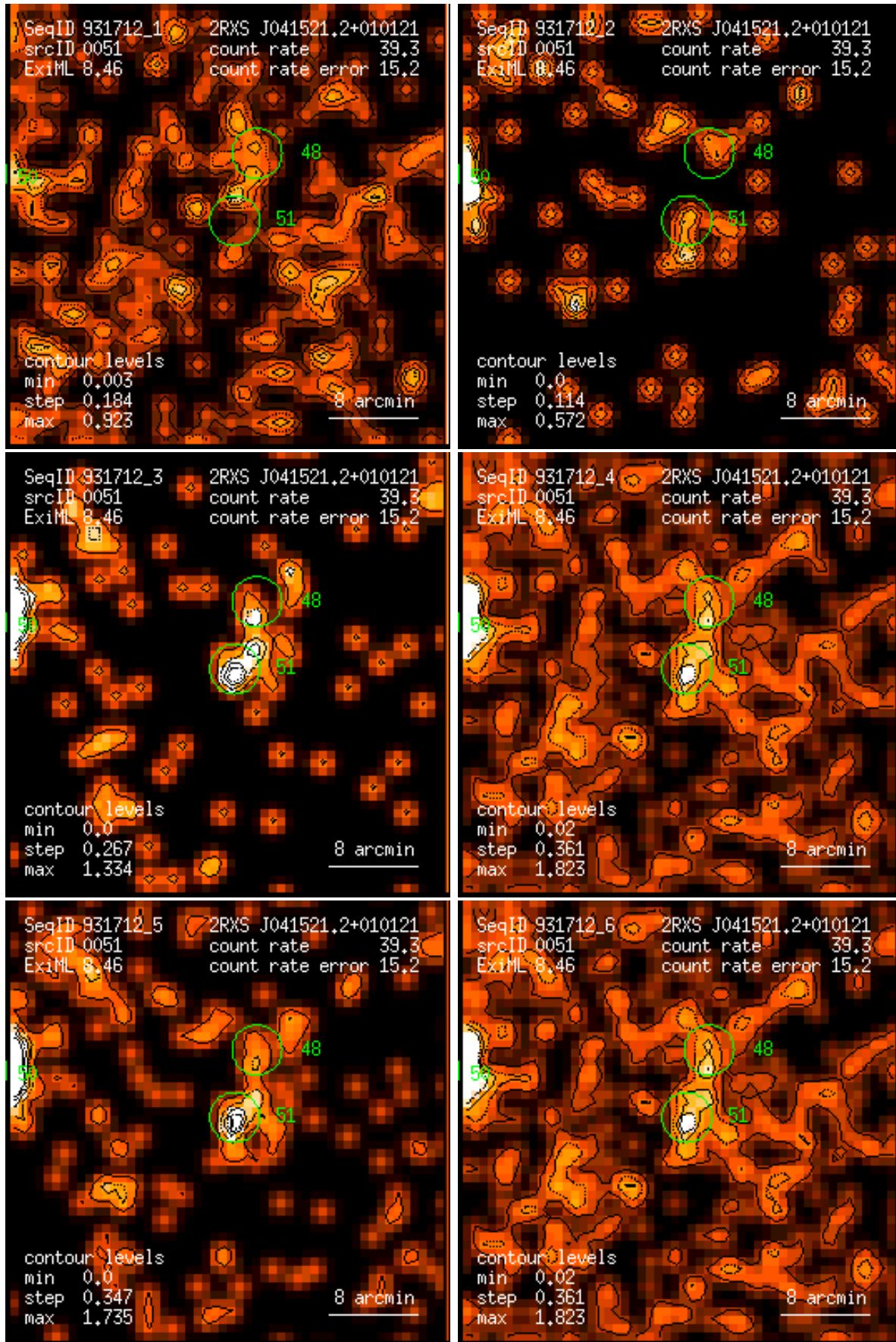
Figure 51: RASS 931712: detection 0051: band rate images, Gaussian filter: (1) PSPC channels 11 – 41, (2) 52 – 90, (3) 91 – 201, (4) 11 – 235, (5) 52 – 201, (6) 11 – 201. Broad band rates in counts/ks. Band rate contour levels in counts/ks/arcmin 2 .
