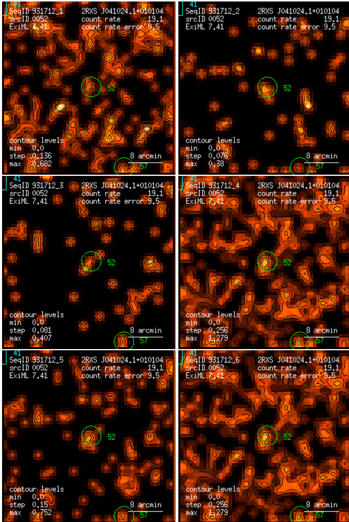
Figure 52: RASS 931712: detection 0052: band rate images, Gaussian filter: (1) PSPC channels 11 – 41, (2) 52 – 90, (3) 91 – 201, (4) 11 – 235, (5) 52 – 201, (6) 11 – 201. Broad band rates in counts/ks. Band rate contour levels in counts/ks/arcmin 2 .
