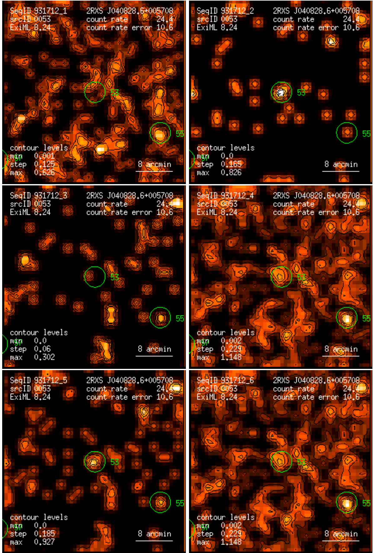
Figure 53: RASS 931712: detection 0053: band rate images, Gaussian filter: (1) PSPC channels 11 – 41, (2) 52 – 90, (3) 91 – 201, (4) 11 – 235, (5) 52 – 201, (6) 11 – 201. Broad band rates in counts/ks. Band rate contour levels in counts/ks/arcmin 2 .
