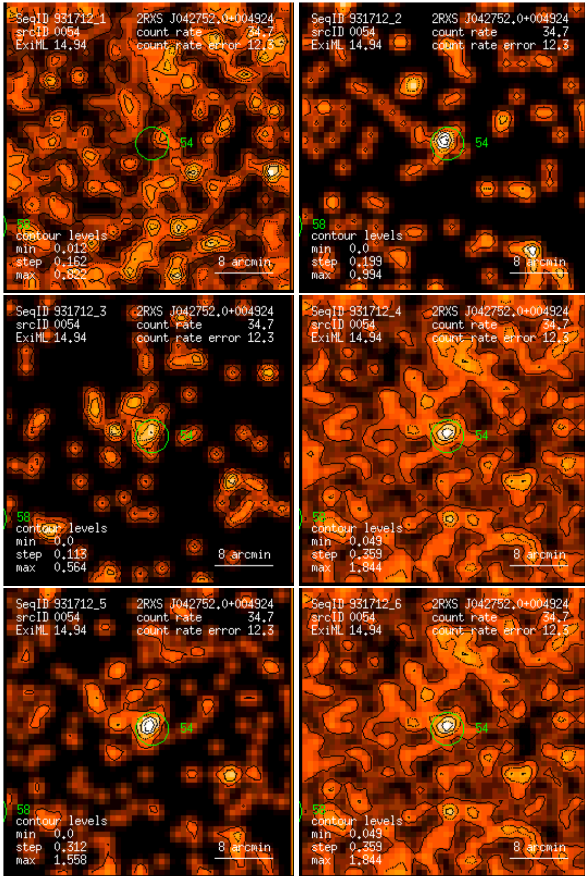
Figure 54: RASS 931712: detection 0054: band rate images, Gaussian filter: (1) PSPC channels 11 – 41, (2) 52 – 90, (3) 91 – 201, (4) 11 – 235, (5) 52 – 201, (6) 11 – 201. Broad band rates in counts/ks. Band rate contour levels in counts/ks/arcmin 2 .
