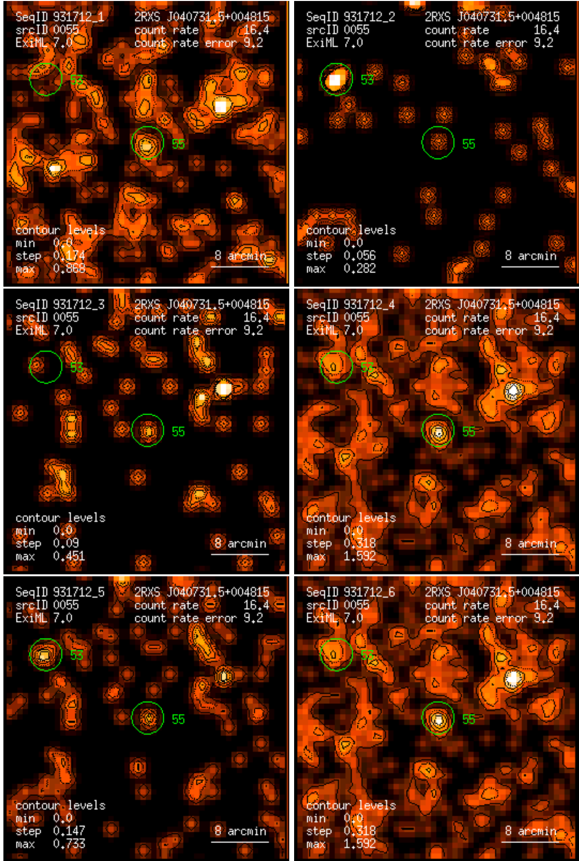
Figure 55: RASS 931712: detection 0055: band rate images, Gaussian filter: (1) PSPC channels 11 – 41, (2) 52 – 90, (3) 91 – 201, (4) 11 – 235, (5) 52 – 201, (6) 11 – 201. Broad band rates in counts/ks. Band rate contour levels in counts/ks/arcmin 2 .
