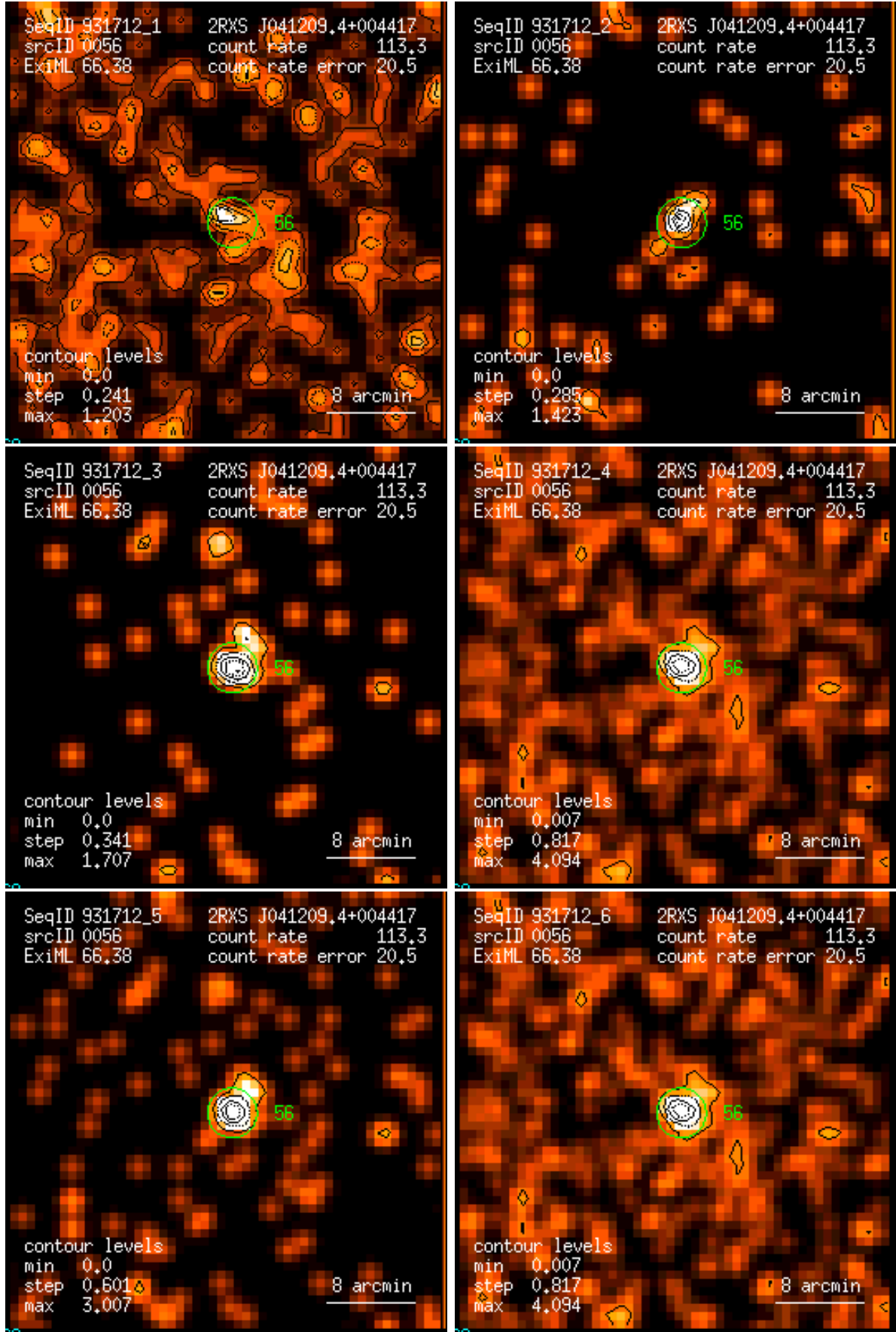
Figure 56: RASS 931712: detection 0056: band rate images, Gaussian filter: (1) PSPC channels 11 – 41, (2) 52 – 90, (3) 91 – 201, (4) 11 – 235, (5) 52 – 201, (6) 11 – 201. Broad band rates in counts/ks. Band rate contour levels in counts/ks/arcmin 2 .
