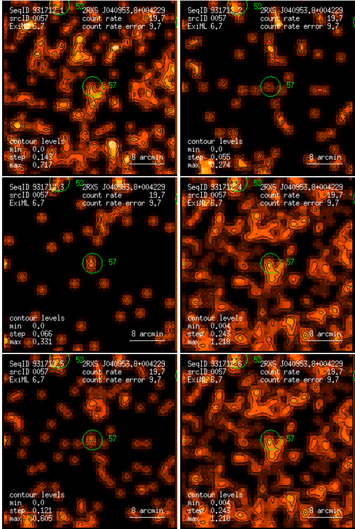
Figure 57: RASS 931712: detection 0057: band rate images, Gaussian filter: (1) PSPC channels 11 – 41, (2) 52 – 90, (3) 91 – 201, (4) 11 – 235, (5) 52 – 201, (6) 11 – 201. Broad band rates in counts/ks. Band rate contour levels in counts/ks/arcmin 2 .
