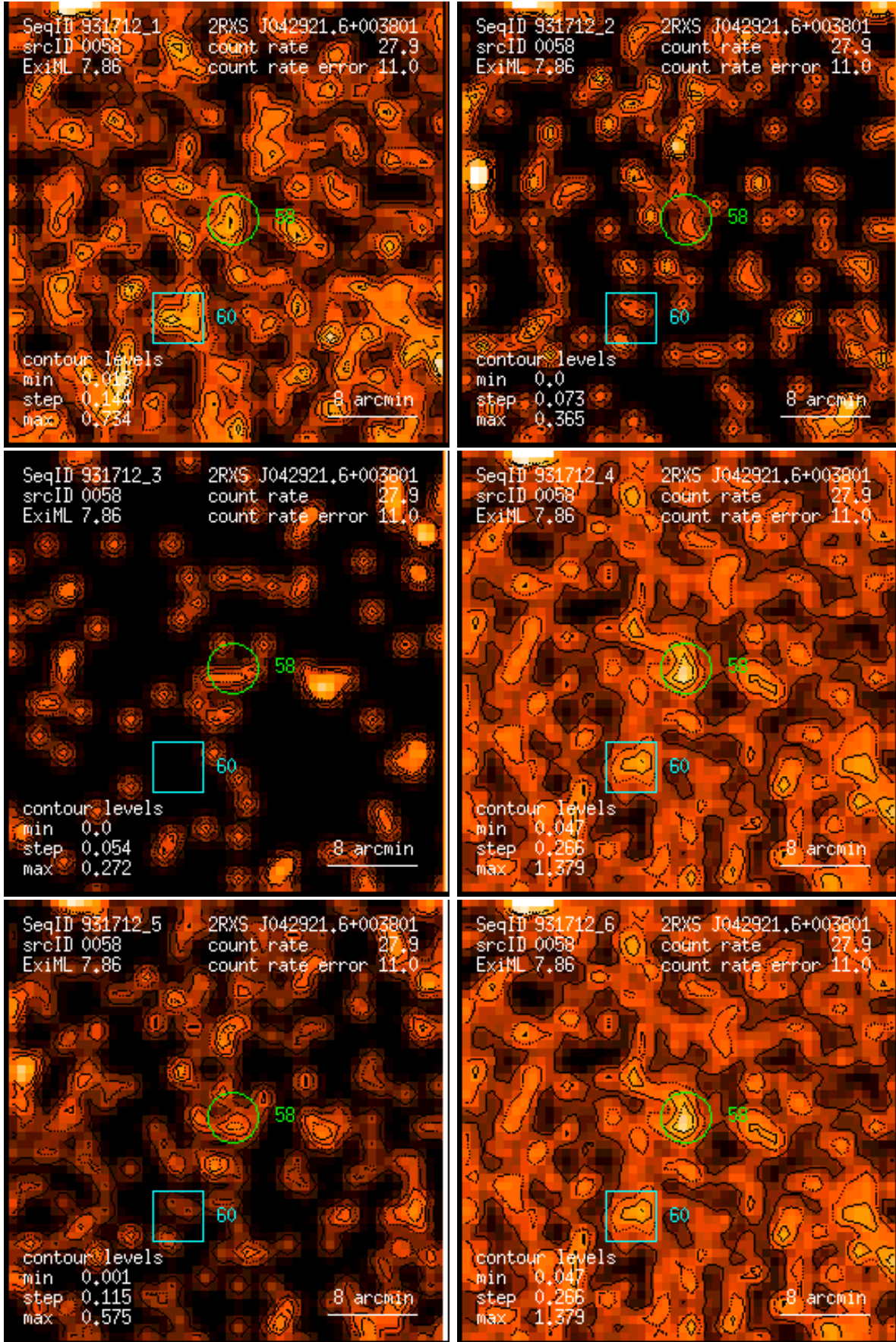
Figure 58: RASS 931712: detection 0058: band rate images, Gaussian filter: (1) PSPC channels 11 – 41, (2) 52 – 90, (3) 91 – 201, (4) 11 – 235, (5) 52 – 201, (6) 11 – 201. Broad band rates in counts/ks. Band rate contour levels in counts/ks/arcmin 2 .
