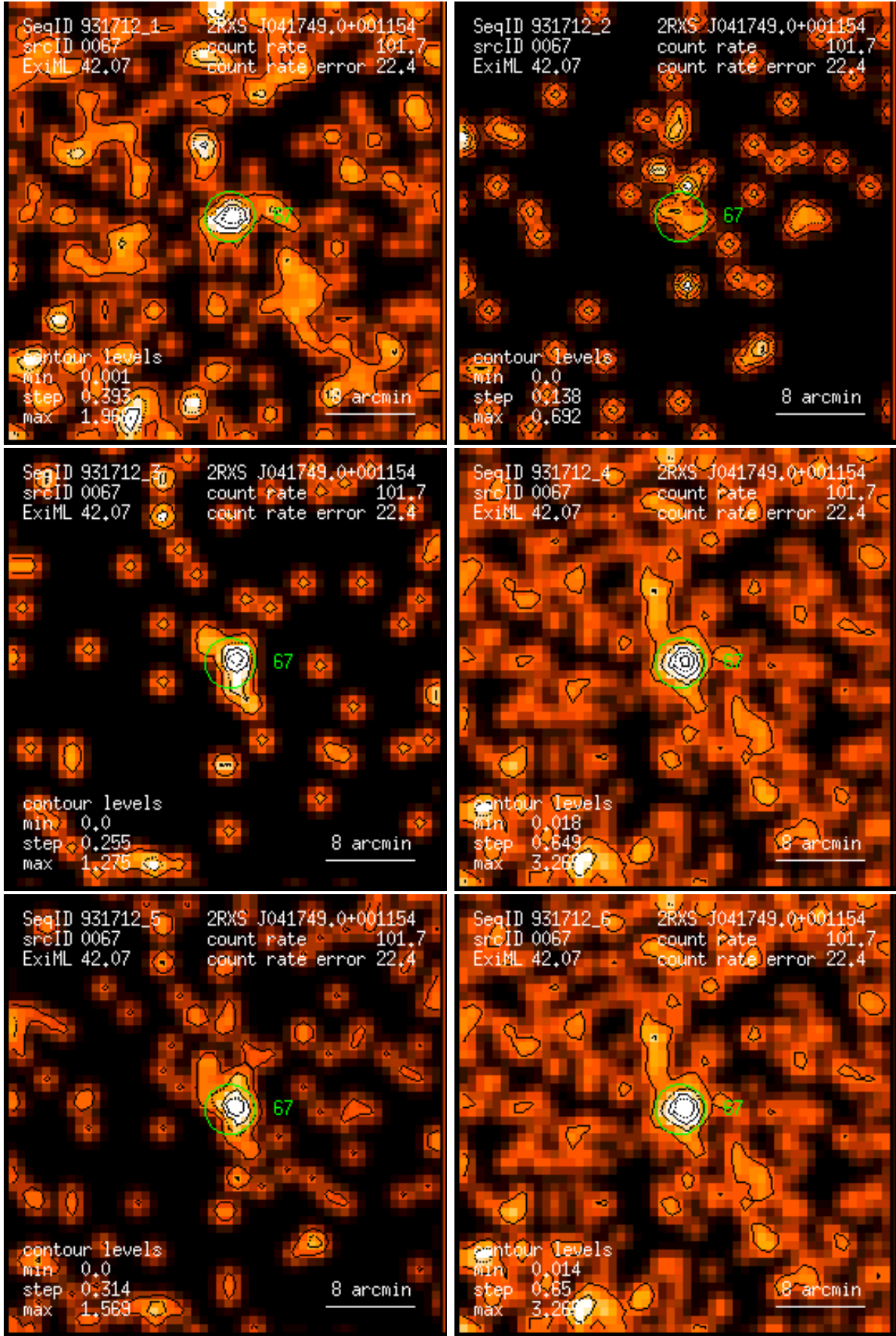
Figure 67: RASS 931712: detection 0067: band rate images, Gaussian filter: (1) PSPC channels 11 – 41, (2) 52 – 90, (3) 91 – 201, (4) 11 – 235, (5) 52 – 201, (6) 11 – 201. Broad band rates in counts/ks. Band rate contour levels in counts/ks/arcmin 2 .
