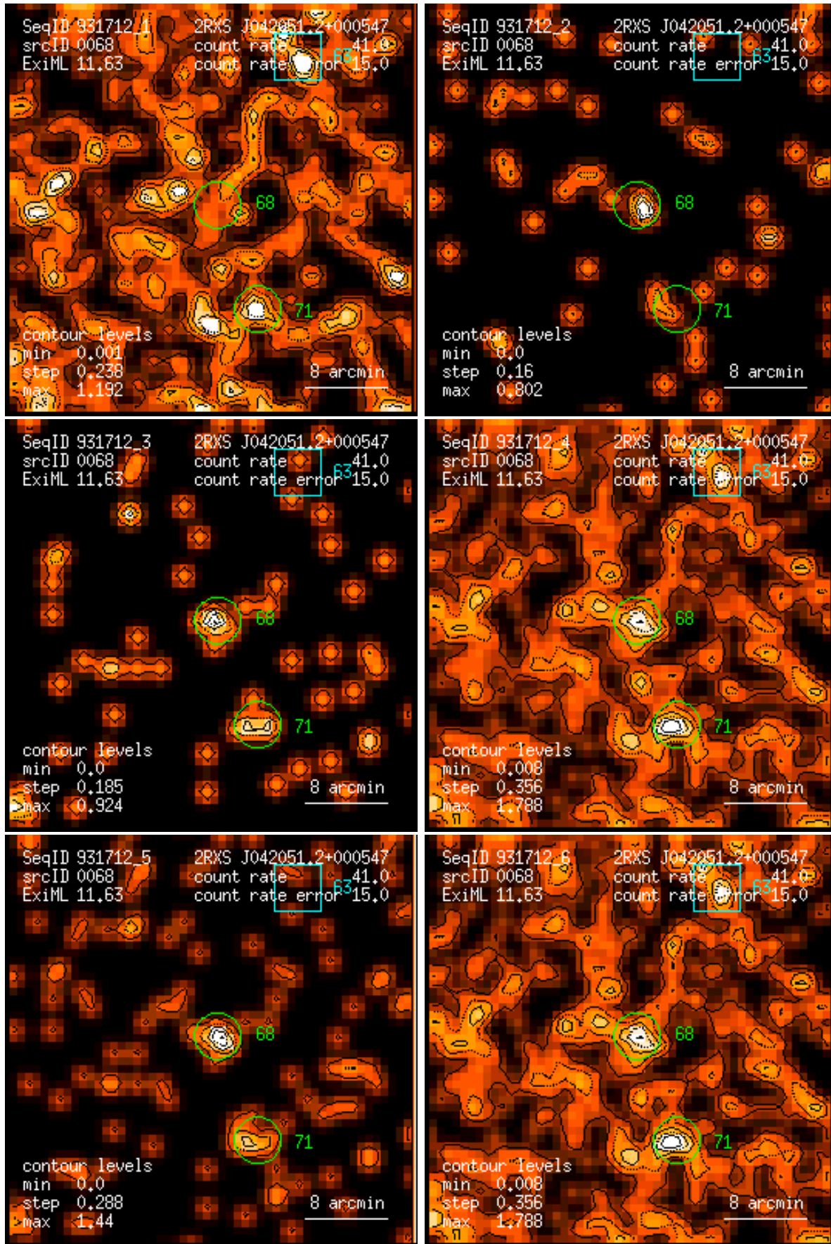
Figure 68: RASS 931712: detection 0068: band rate images, Gaussian filter: (1) PSPC channels 11 – 41, (2) 52 – 90, (3) 91 – 201, (4) 11 – 235, (5) 52 – 201, (6) 11 – 201. Broad band rates in counts/ks. Band rate contour levels in counts/ks/arcmin 2 .
