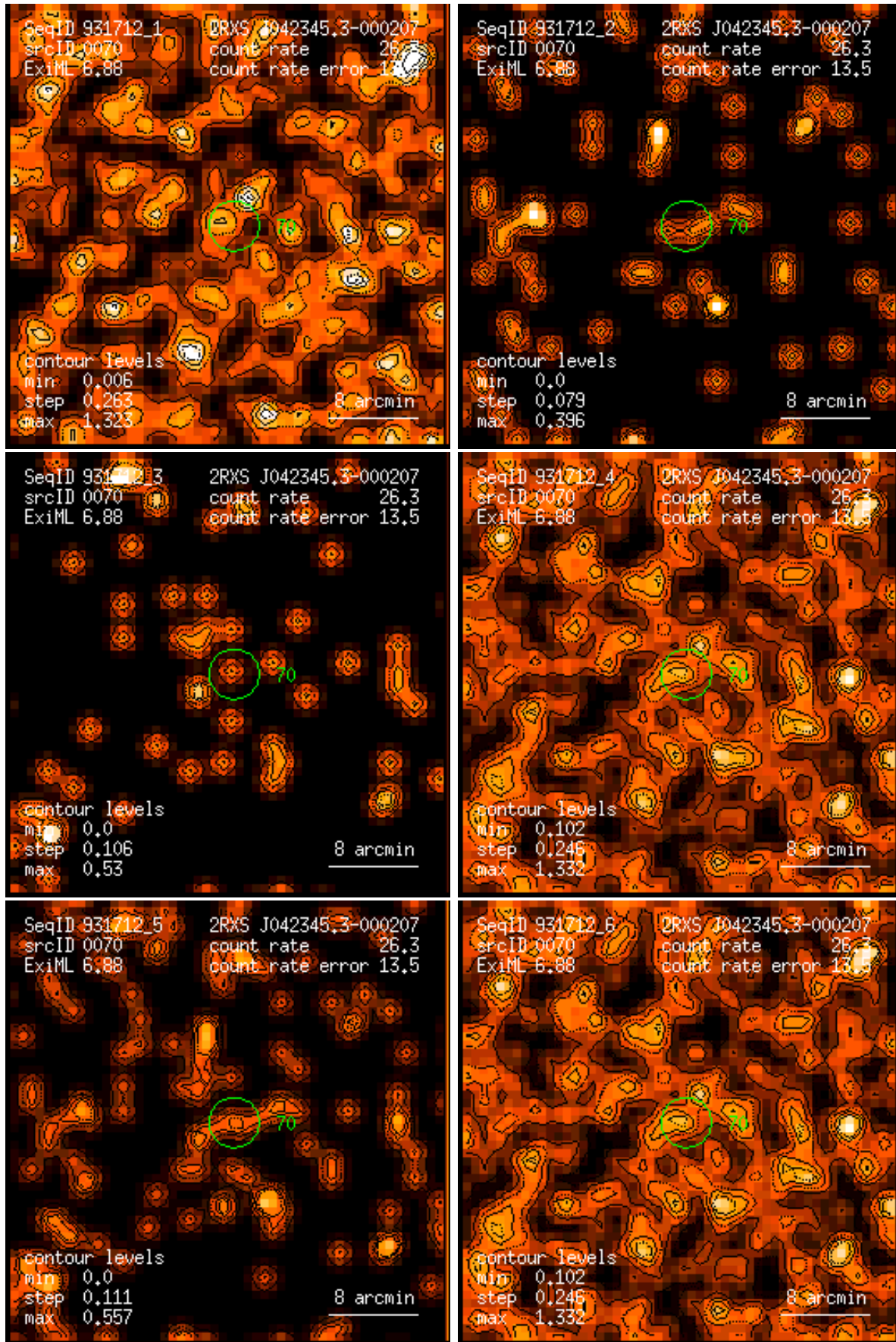
Figure 70: RASS 931712: detection 0070: band rate images, Gaussian filter: (1) PSPC channels 11 – 41, (2) 52 – 90, (3) 91 – 201, (4) 11 – 235, (5) 52 – 201, (6) 11 – 201. Broad band rates in counts/ks. Band rate contour levels in counts/ks/arcmin 2 .
