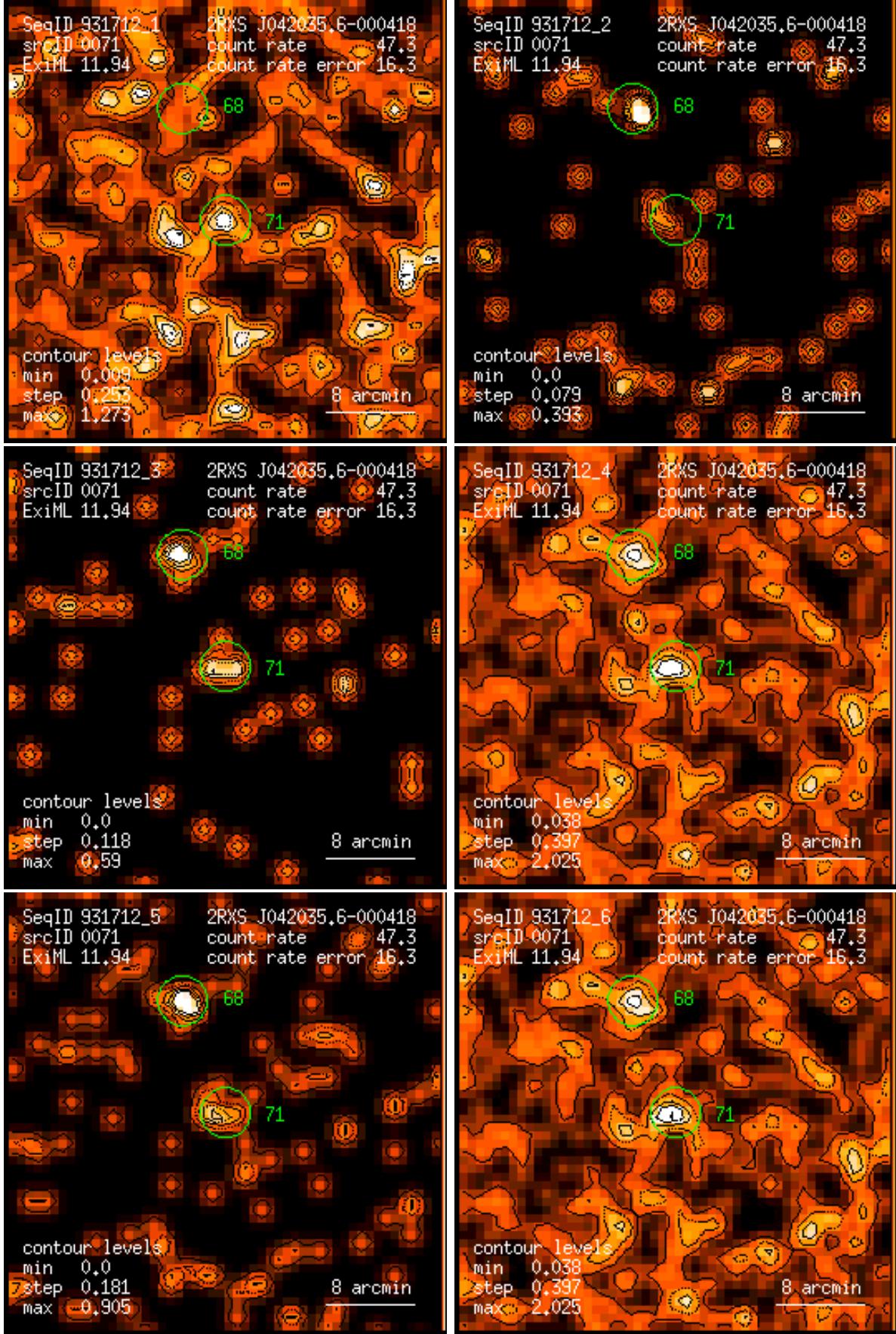
Figure 71: RASS 931712: detection 0071: band rate images, Gaussian filter: (1) PSPC channels 11 – 41, (2) 52 – 90, (3) 91 – 201, (4) 11 – 235, (5) 52 – 201, (6) 11 – 201. Broad band rates in counts/ks. Band rate contour levels in counts/ks/arcmin 2 .
