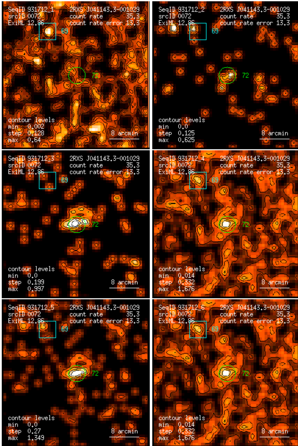
Figure 72: RASS 931712: detection 0072: band rate images, Gaussian filter: (1) PSPC channels 11 – 41, (2) 52 – 90, (3) 91 – 201, (4) 11 – 235, (5) 52 – 201, (6) 11 – 201. Broad band rates in counts/ks. Band rate contour levels in counts/ks/arcmin 2 .
