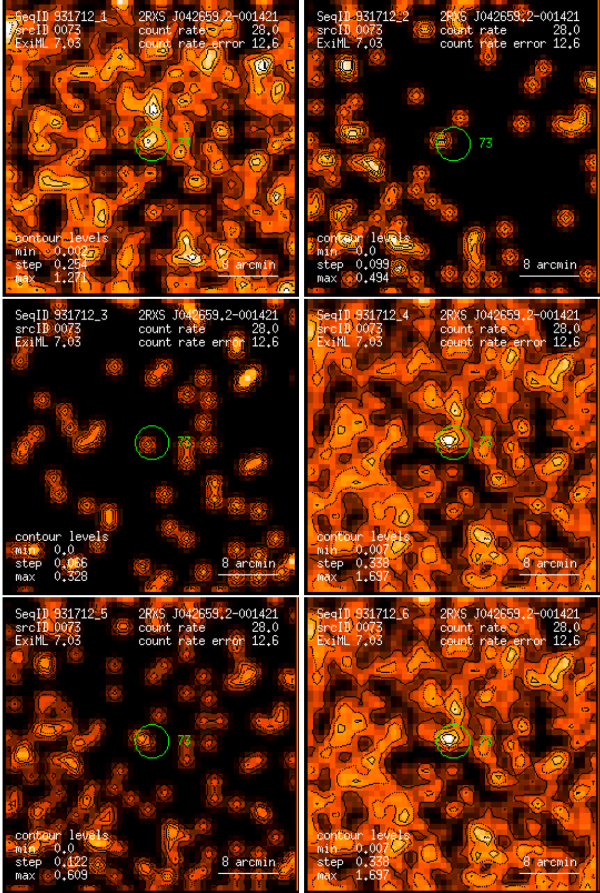
Figure 73: RASS 931712: detection 0073: band rate images, Gaussian filter: (1) PSPC channels 11 – 41, (2) 52 – 90, (3) 91 – 201, (4) 11 – 235, (5) 52 – 201, (6) 11 – 201. Broad band rates in counts/ks. Band rate contour levels in counts/ks/arcmin 2 .
