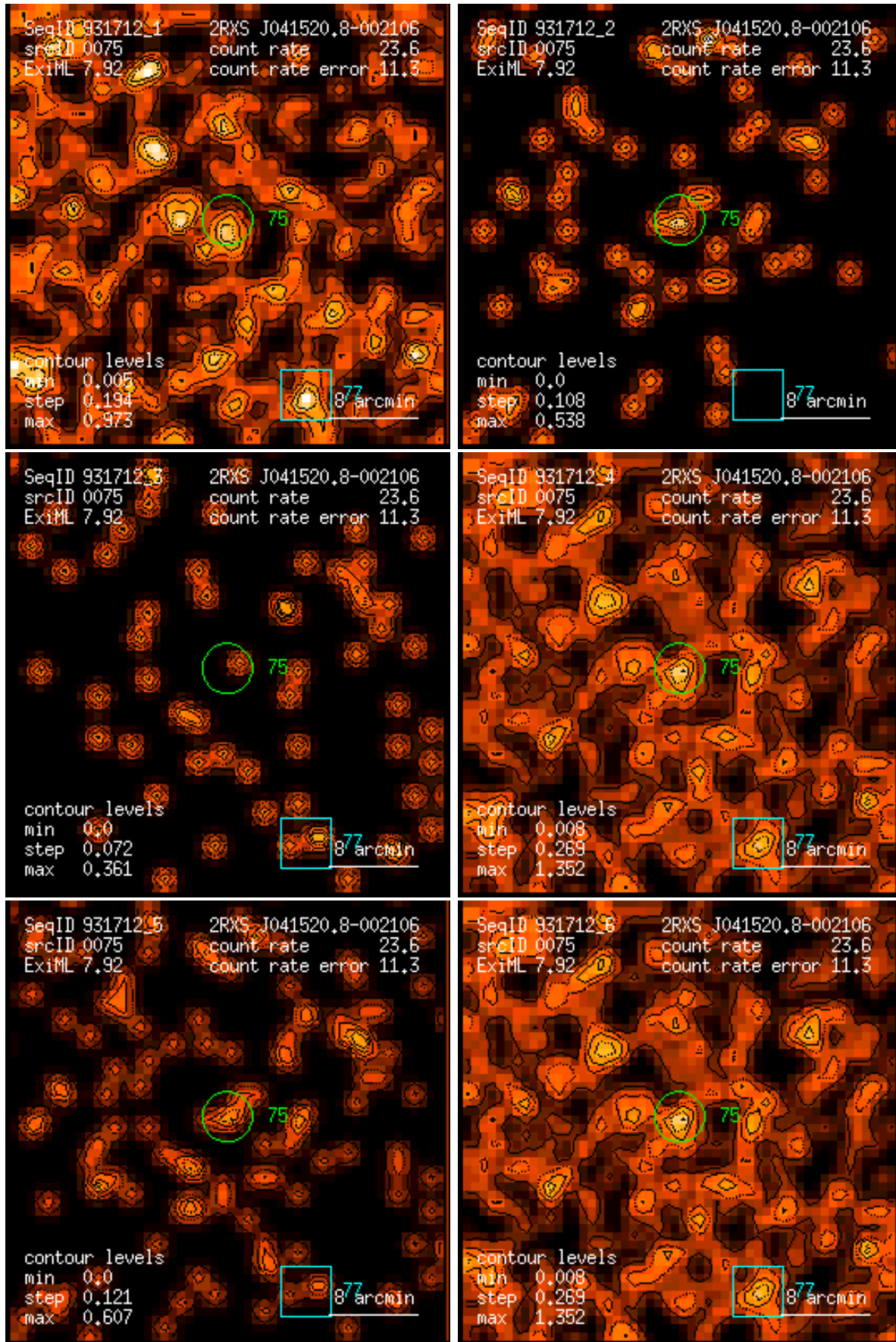
Figure 75: RASS 931712: detection 0075: band rate images, Gaussian filter: (1) PSPC channels 11 – 41, (2) 52 – 90, (3) 91 – 201, (4) 11 – 235, (5) 52 – 201, (6) 11 – 201. Broad band rates in counts/ks. Band rate contour levels in counts/ks/arcmin 2 .
