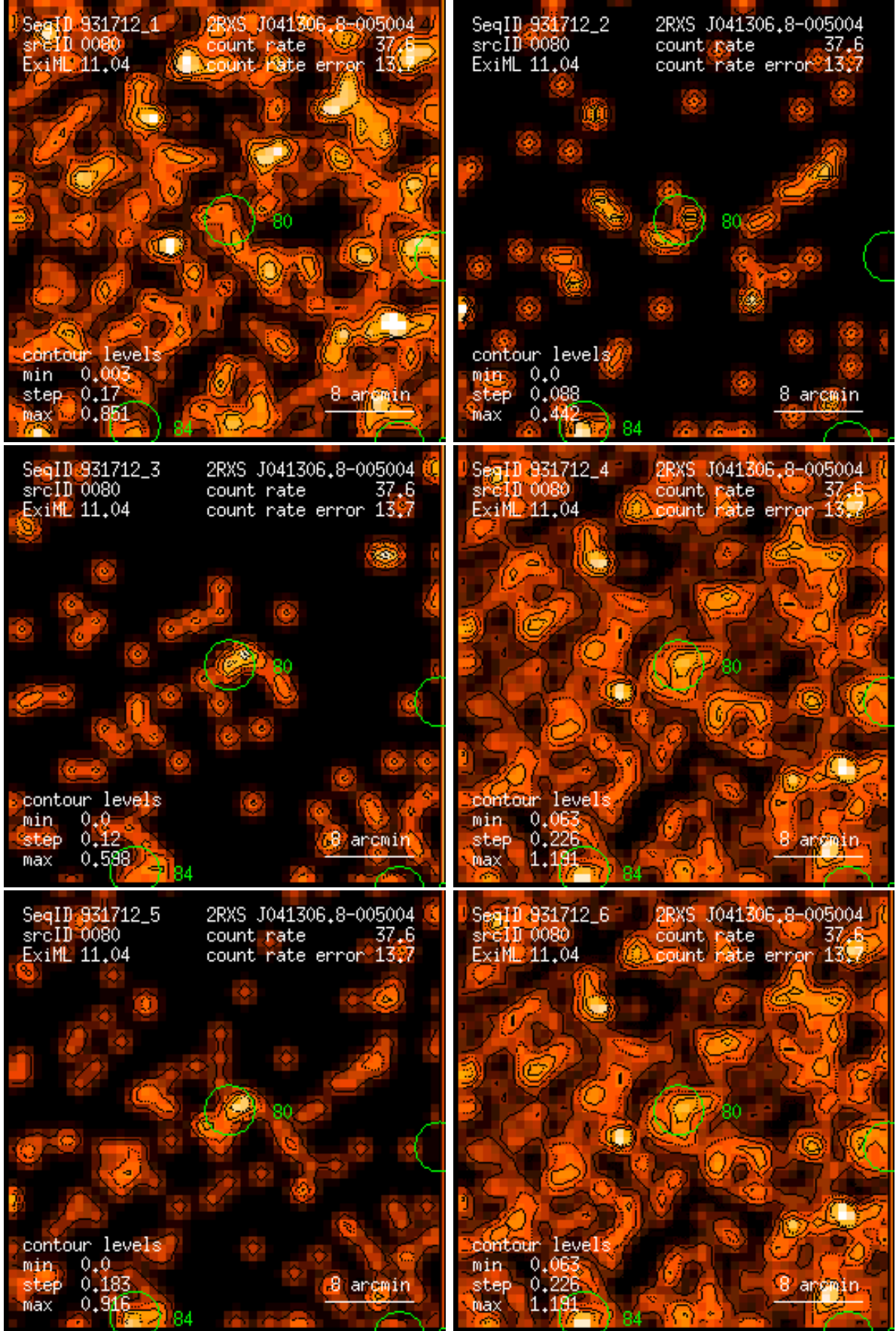
Figure 80: RASS 931712: detection 0080: band rate images, Gaussian filter: (1) PSPC channels 11 – 41, (2) 52 – 90, (3) 91 – 201, (4) 11 – 235, (5) 52 – 201, (6) 11 – 201. Broad band rates in counts/ks. Band rate contour levels in counts/ks/arcmin 2 .
