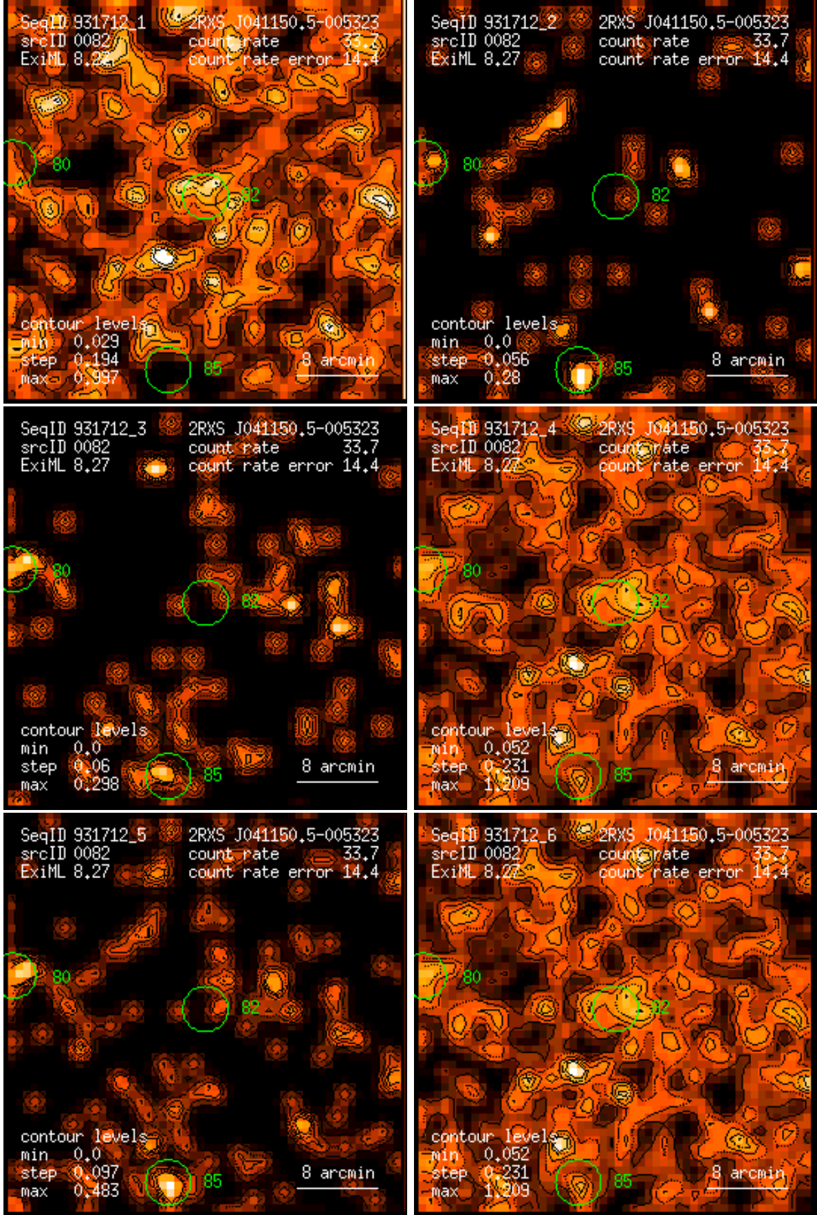
Figure 82: RASS 931712: detection 0082: band rate images, Gaussian filter: (1) PSPC channels 11 – 41, (2) 52 – 90, (3) 91 – 201, (4) 11 – 235, (5) 52 – 201, (6) 11 – 201. Broad band rates in counts/ks. Band rate contour levels in counts/ks/arcmin 2 .
