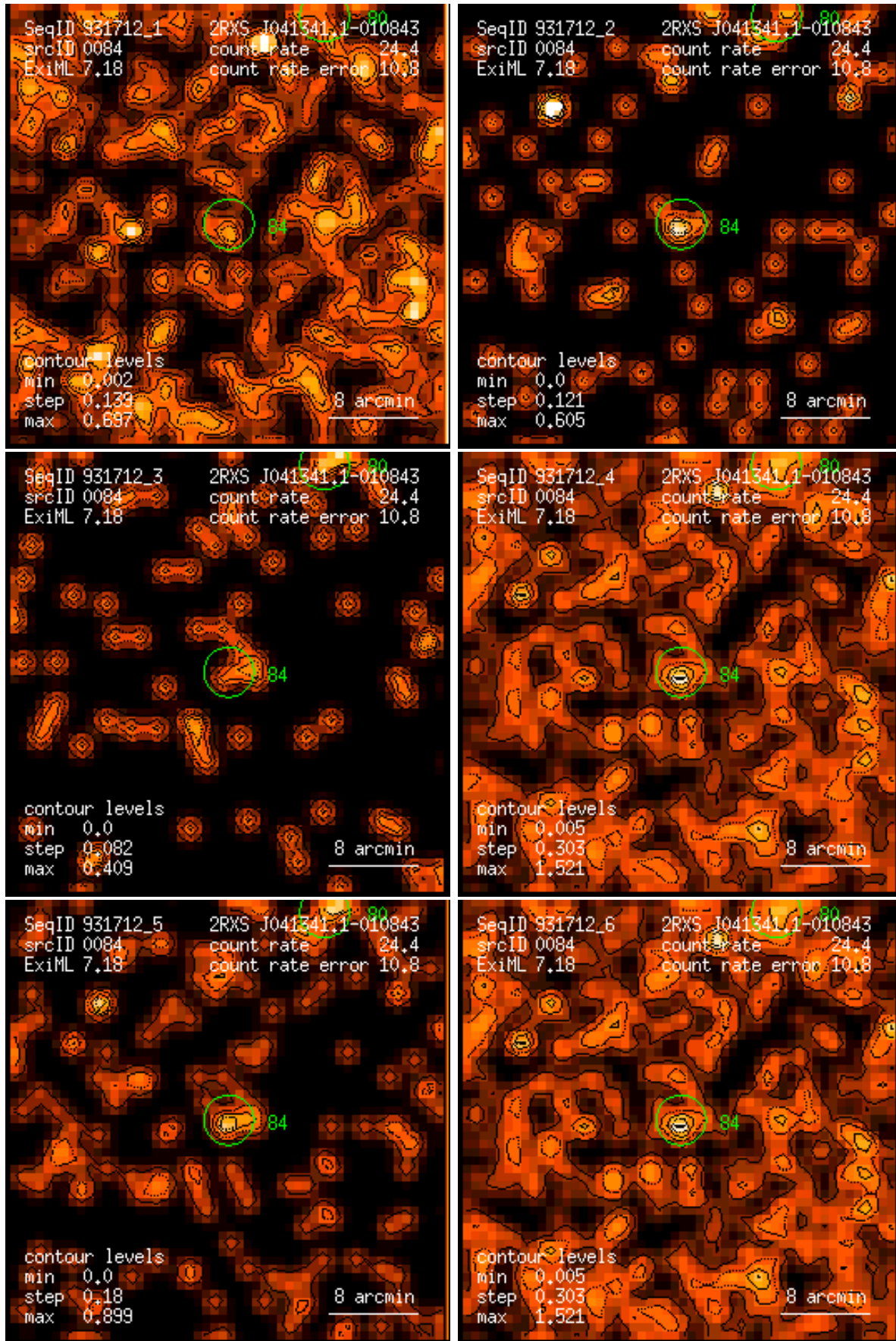
Figure 84: RASS 931712: detection 0084: band rate images, Gaussian filter: (1) PSPC channels 11 – 41, (2) 52 – 90, (3) 91 – 201, (4) 11 – 235, (5) 52 – 201, (6) 11 – 201. Broad band rates in counts/ks. Band rate contour levels in counts/ks/arcmin 2 .
