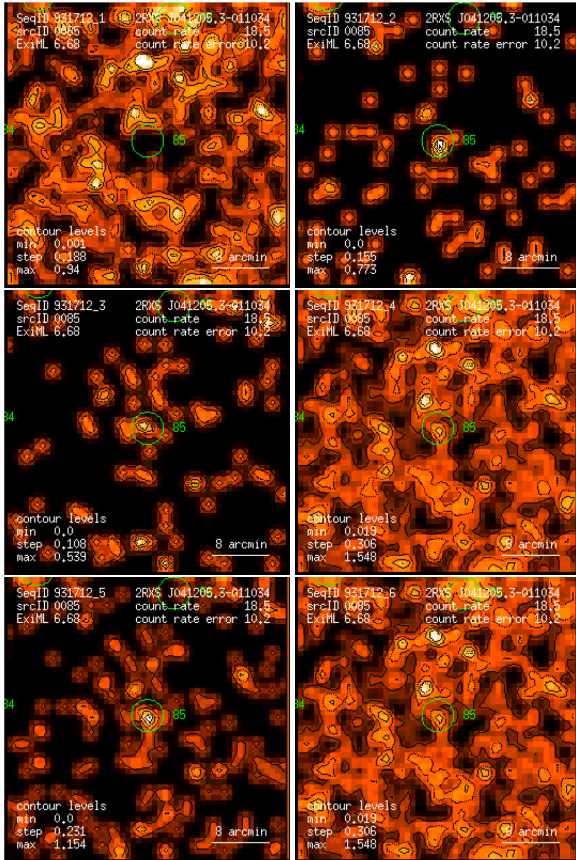
Figure 85: RASS 931712: detection 0085: band rate images, Gaussian filter: (1) PSPC channels 11 – 41, (2) 52 – 90, (3) 91 – 201, (4) 11 – 235, (5) 52 – 201, (6) 11 – 201. Broad band rates in counts/ks. Band rate contour levels in counts/ks/arcmin 2 .
