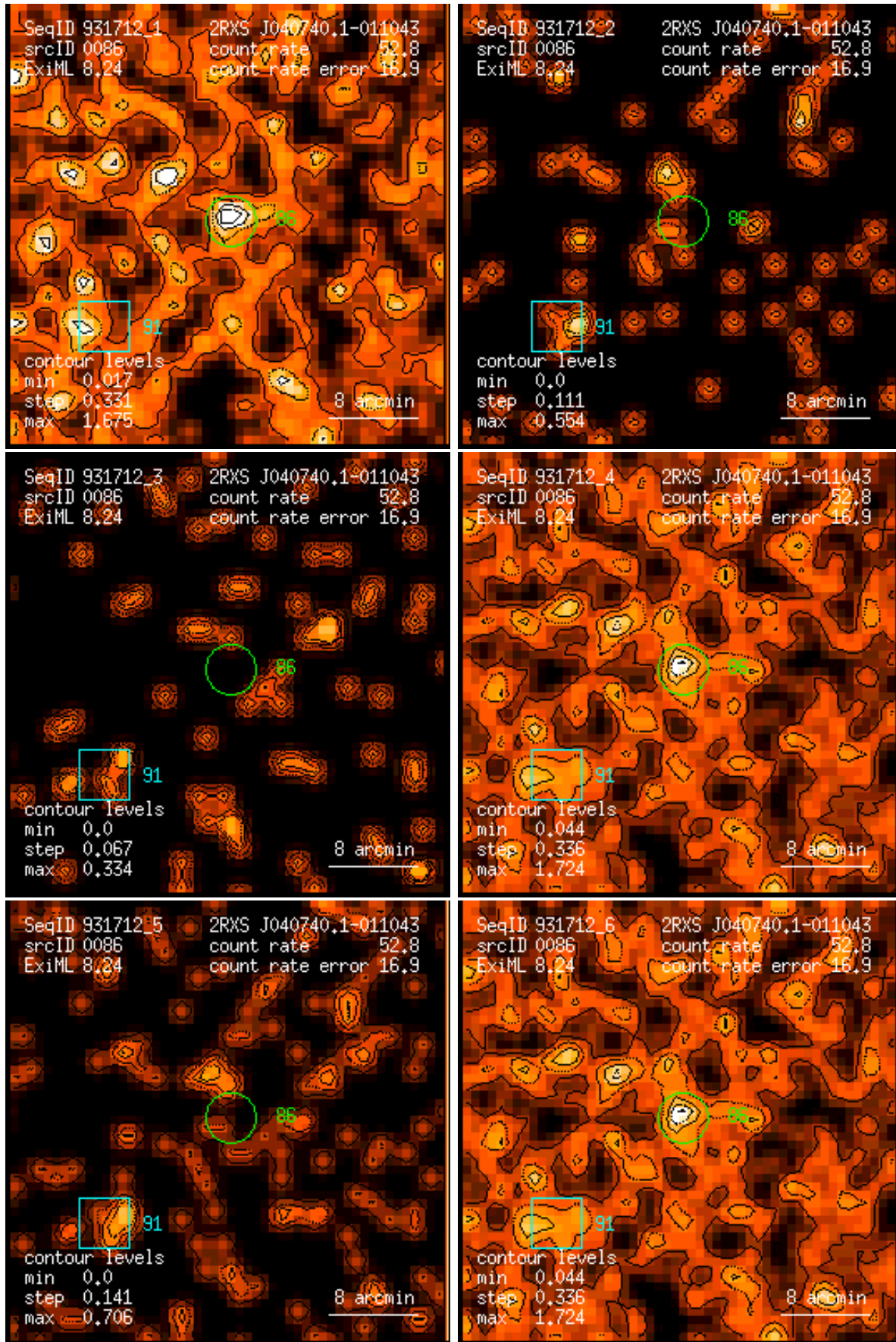
Figure 86: RASS 931712: detection 0086: band rate images, Gaussian filter: (1) PSPC channels 11 – 41, (2) 52 – 90, (3) 91 – 201, (4) 11 – 235, (5) 52 – 201, (6) 11 – 201. Broad band rates in counts/ks. Band rate contour levels in counts/ks/arcmin 2 .
