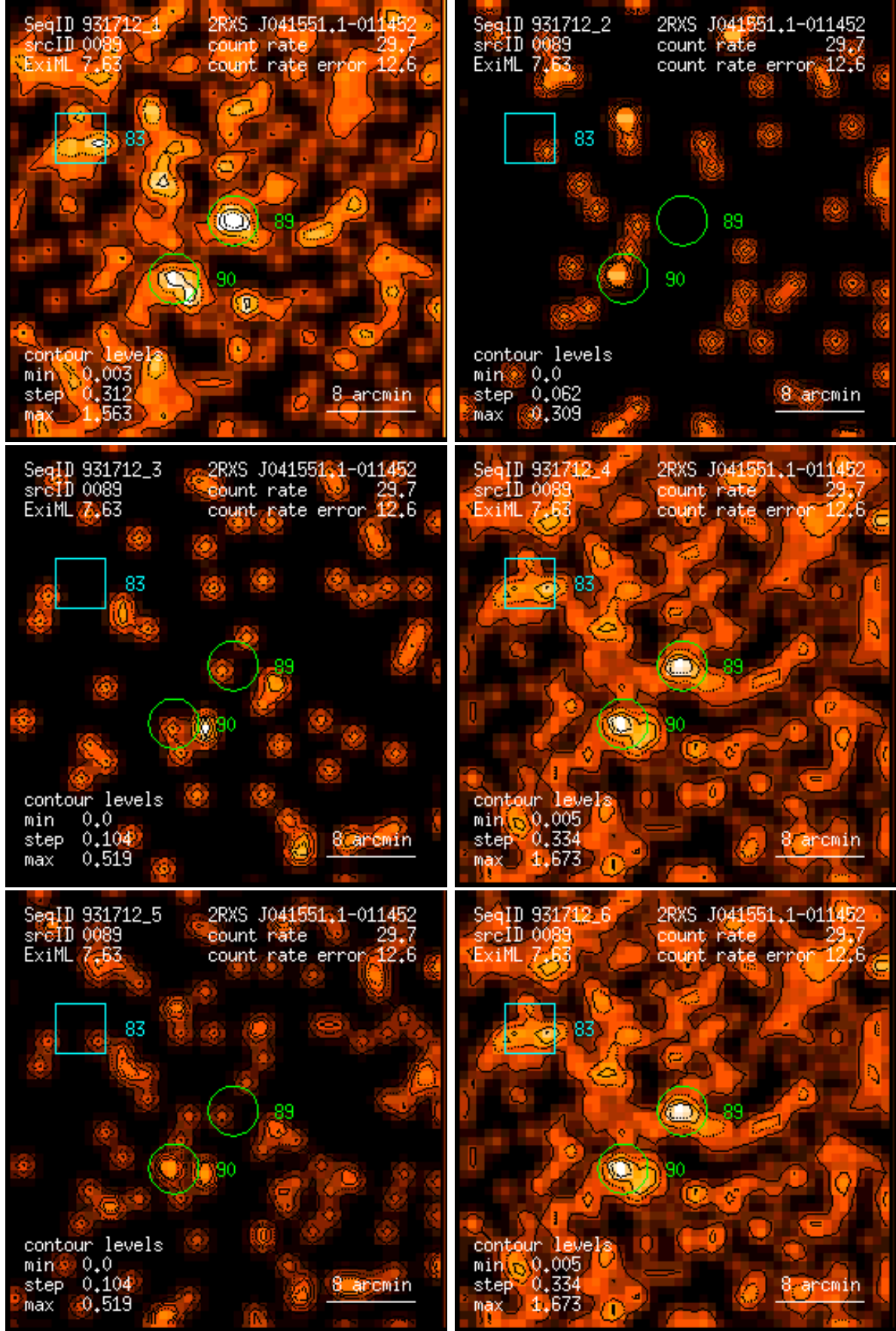
Figure 89: RASS 931712: detection 0089: band rate images, Gaussian filter: (1) PSPC channels 11 – 41, (2) 52 – 90, (3) 91 – 201, (4) 11 – 235, (5) 52 – 201, (6) 11 – 201. Broad band rates in counts/ks. Band rate contour levels in counts/ks/arcmin 2 .
