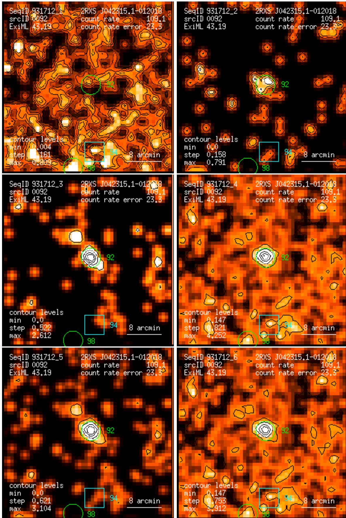
Figure 92: RASS 931712: detection 0092: band rate images, Gaussian filter: (1) PSPC channels 11 – 41, (2) 52 – 90, (3) 91 – 201, (4) 11 – 235, (5) 52 – 201, (6) 11 – 201. Broad band rates in counts/ks. Band rate contour levels in counts/ks/arcmin 2 .
