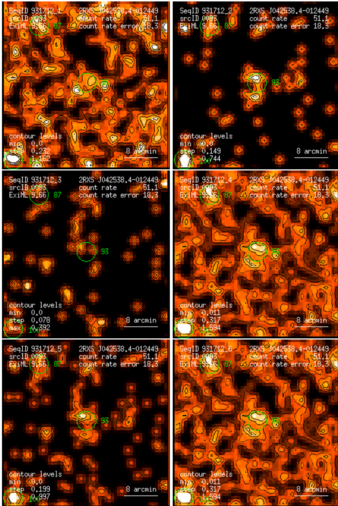
Figure 93: RASS 931712: detection 0093: band rate images, Gaussian filter: (1) PSPC channels 11 – 41, (2) 52 – 90, (3) 91 – 201, (4) 11 – 235, (5) 52 – 201, (6) 11 – 201. Broad band rates in counts/ks. Band rate contour levels in counts/ks/arcmin 2 .
