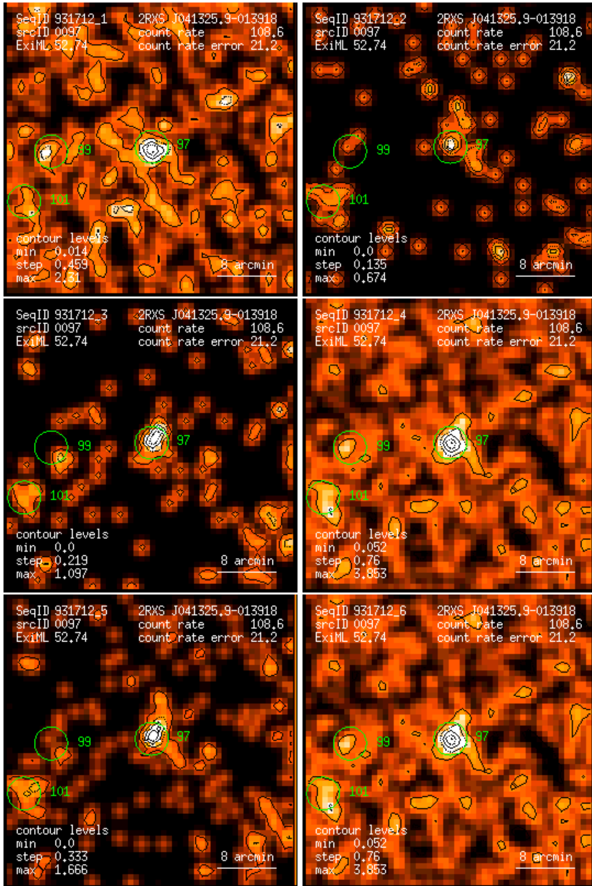
Figure 97: RASS 931712: detection 0097: band rate images, Gaussian filter: (1) PSPC channels 11 – 41, (2) 52 – 90, (3) 91 – 201, (4) 11 – 235, (5) 52 – 201, (6) 11 – 201. Broad band rates in counts/ks. Band rate contour levels in counts/ks/arcmin 2 .
